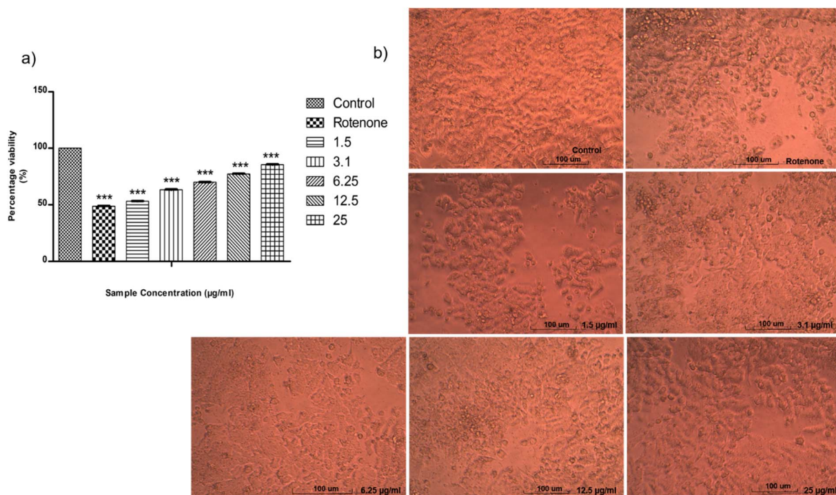
Fig. 6 (a) Graphical representation depicting the neuroprotective effect of ISB1 on SH-SY5Y cells by MTT assay. Co-treatment with ISB1 attenuated vulnerability of SH-SY5Y to rotenone. (b) The morphology changes of the cells.
