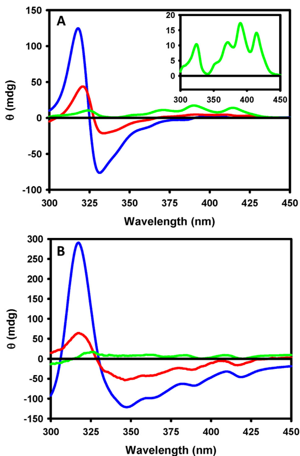
Figure 3. Circular dichroism spectra of alkyl esters of L-Ascorbic Acid (ASC n )/AmB formulation at pH 8 (A) or pH 4 (B). The spectra correspond to AmB with ASC n in aqueous suspension: ascorbyl palmitate (ASC16) (green), ascorbyl myristate (ASC14) (red) and ascorbyl laurate (ASC12) (blue) formulations. AmB concentration was 20.4 μM. The inset in A shows an amplified section of ASC16/AmB spectrum.
