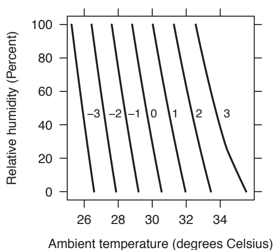
Fig. i. Predicted mean vote against temperature and relative humidity. Plot of the predicted mean vote (PMV) of a large group of naked resting subjects about thermal comfort according to a psycho-physical scale (+3 = hot, +2 = warm, +1 = slightly warm, 0 = neutral, -1 = slightly cool, -2 = cool, -3 = cold) depending on relative humidity and ambient temperature, with only convection current, inside, at sea level [26,27].
