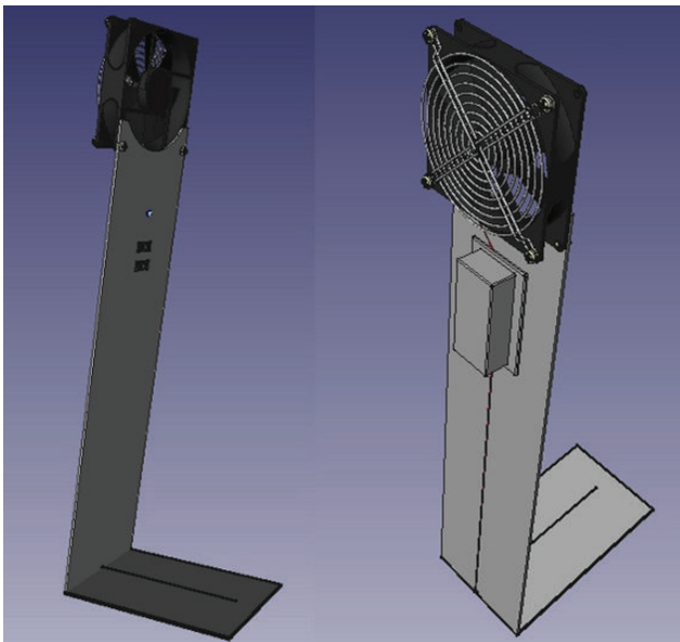
Figure 1. A computer box fan (in this design with dimensions 12 \times 12 \times 2.5 cm) is mounted on a pedestal, which makes a ten degree angle with the floor surface, for stability and for blowing air slightly downward. In this design, the pedestal has a LED light with separate switch.
