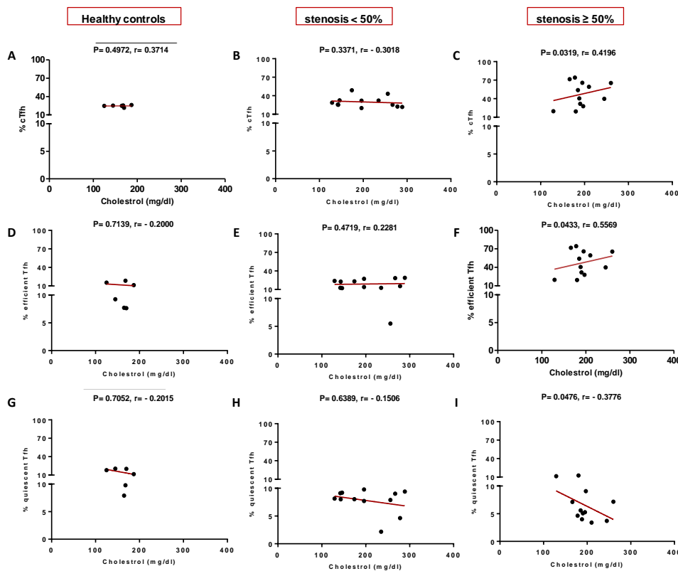
Fig. 8. Correlation of the percentage of cTfh (A and C), efficient (D and F) and quiescent (G and I) cells with Cholesterol in all the three groups (Spearman's rank correlation).
