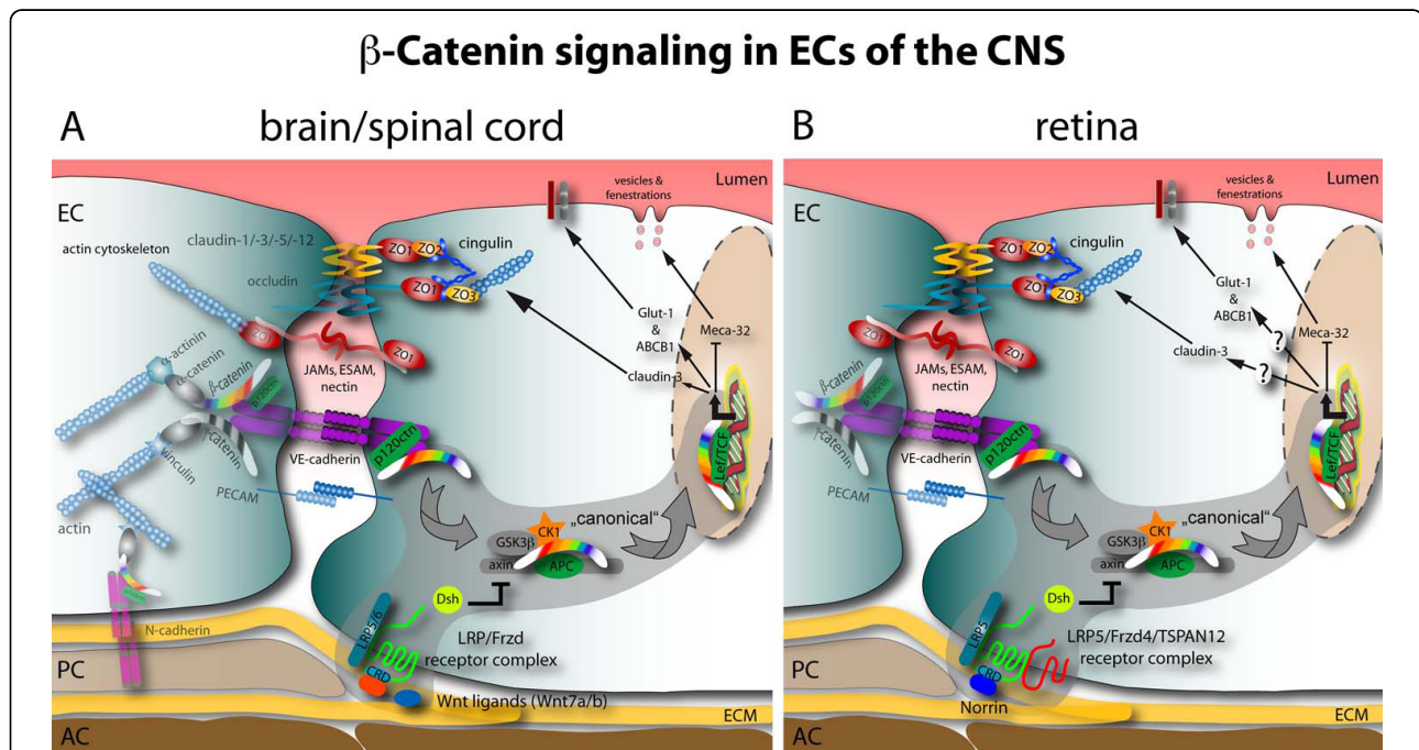
Figure 1 Schematic junctional organization and β-catenin signaling in CNS ECs: comparison of brain and retina. A In the brain and spinal cord mainly Wnt7a and Wnt7b growth factors act on an uncharacterized Fzd-LRP receptor complex to elicit β-catenin target gene transcription. The positively regulated target genes identified so far are the TJ protein claudin-3, Glut-1 and ABCB1/MDR1. Conversely, the expression of Meca-32/Plvap becomes suppressed by β-catenin transcription via an unknown mechanism. B in the retina Norrin is the predominant ligand activating β-catenin signaling downstream of the Fzd4-LRP5-TSPAN12 receptor complex. So far only the repression of Meca-32/Plvap was identified as target of this signaling. To date the effect of Norrin signaling on claudin-3, Glut-1 or other barrier-related genes is not know. See the grey supported area and arrows for the “canonical” Wnt pathway.
