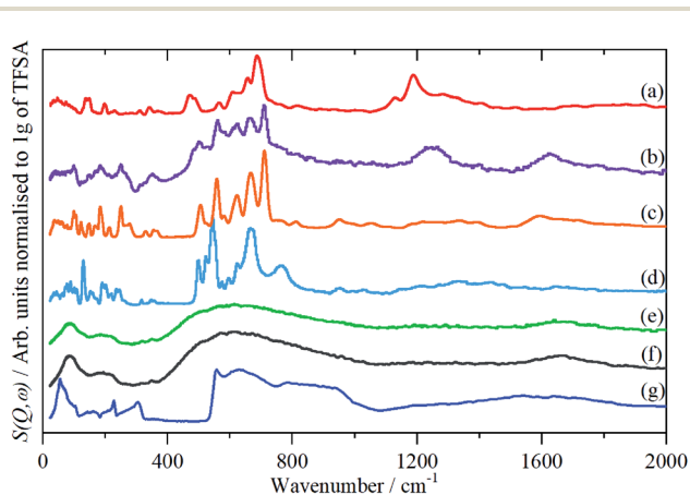
Fig. 5 INS (TOSCA) spectra of \text{TFSA}\cdot n\text{H}_2\text{O} at <20\text{ K} : (a) n = 0 , (b) n = 0.5 , (c) n = 1 , (d) n = 2 , (e) n = 4 , (f) n = 5 , (g) ice I_h . Relative to (d), (e) and (f); (a) is \times 6 , (b) is \times 3 and (c) \times 2 ordinate expanded.
