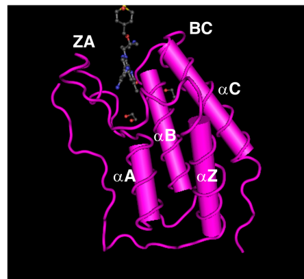
Figure 2. The tertiary structure of the human BRD4-BDI complex with the inhibitor JQ1. A long loop (loop ZA) connects helices \alpha Z and \alpha A , and another loop (loop BC) connects helices \alpha B and \alpha C . A pocket-shaped region formed by these two loops is a binding site for JQ1 or an acetylated lysine residue in histones. The small molecule seen in the pocket is the inhibitor JQ1. The structure of BRD4-BDI is based on the NCBI database information provided in the accession number 3MXF_A.
