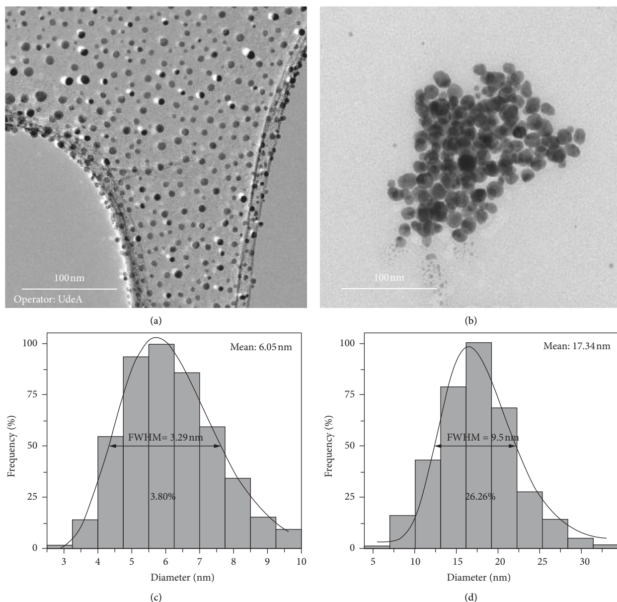
FIGURE 3: TEM micrograph of silver nanoparticles. (a) AgNPs obtained by “green” synthesis. (b) AgNPs obtained by the nongreen method. Differential size distribution of (c) G-AgNPs and (d) S-AgNPs.
