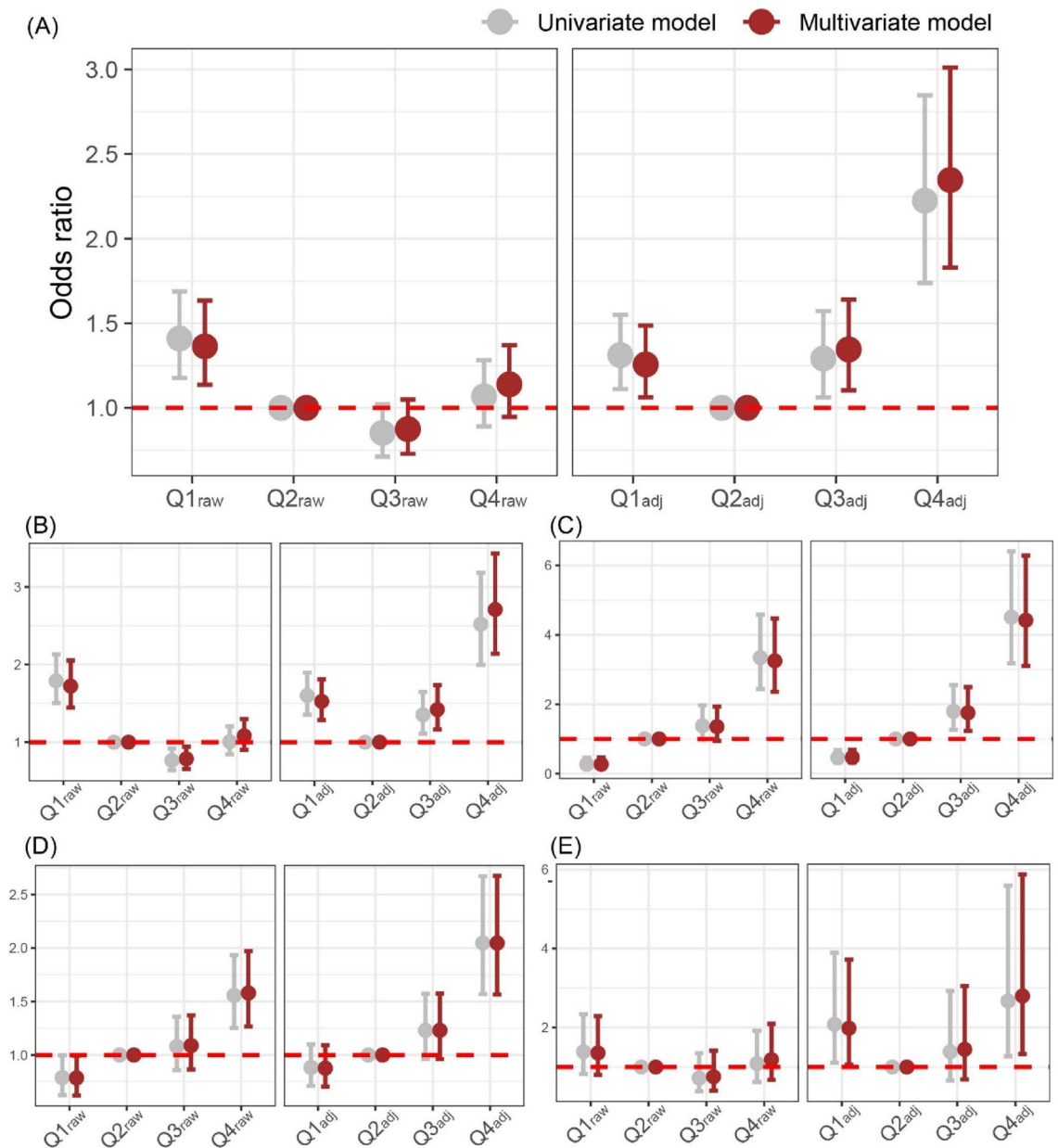
Figure 4. Logistic regression. Q2 raw and Q2 adj were used as references in all models. Age, hypertension, diabetes, and parity types are covariates for multivariate models. Logistic regression method was used to reveal the relationship between main outcome and four groups based on serum creatinine measurements. Relationship of the four SCr groups with all types of adverse pregnancy outcomes (A), preterm birth (B), preeclampsia (C), fetal growth retardation (D), and intrauterine fetal demise (E) are illustrated.
