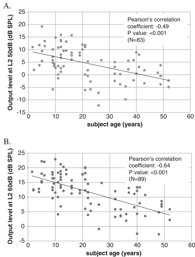
Figure 1 DPOAE ( 2f_1-f_2 ) amplitude as a function of age. In the upper plot (A) stimulus level L_2 = 50 dB SPL. In lower graph (B) stimulus L_2 = 60 dB SPL. Pearson's correlation coefficients and statistical significance values are indicated.
