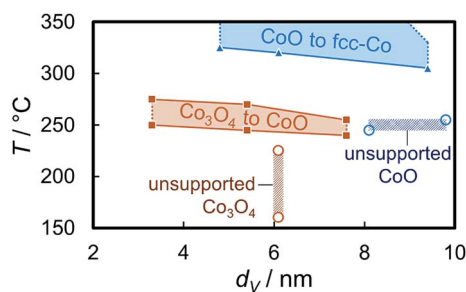
Fig. 10 Temperature ranges for a 1\text{ °C min}^{-1} ramp rate of the reduction of exfoliated graphite-supported (5 wt% Co) and unsupported \text{Co}_3\text{O}_4 crystallites to CoO and the subsequent reduction to metallic Co in hydrogen as observed via in situ X-ray diffraction as a function of the volume-mean crystallite size as obtained from Rietveld refinement.
