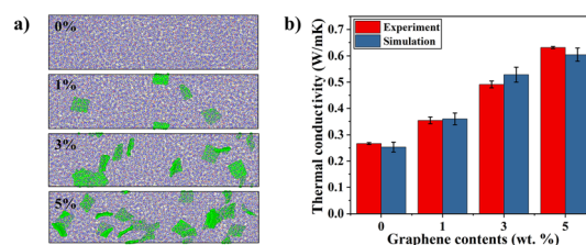
Fig. 3 (a) Molecular structure model of randomly distributed graphene/PEEK nanocomposites with different graphene contents (0 wt%, 1 wt%, 3 wt%, 5 wt%); (b) molecular dynamics simulation of different graphene contents compared with experimental results of TC.
