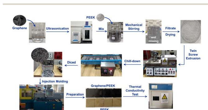
Fig. 2 PEEK and graphene/PEEK preparation flow chart.
