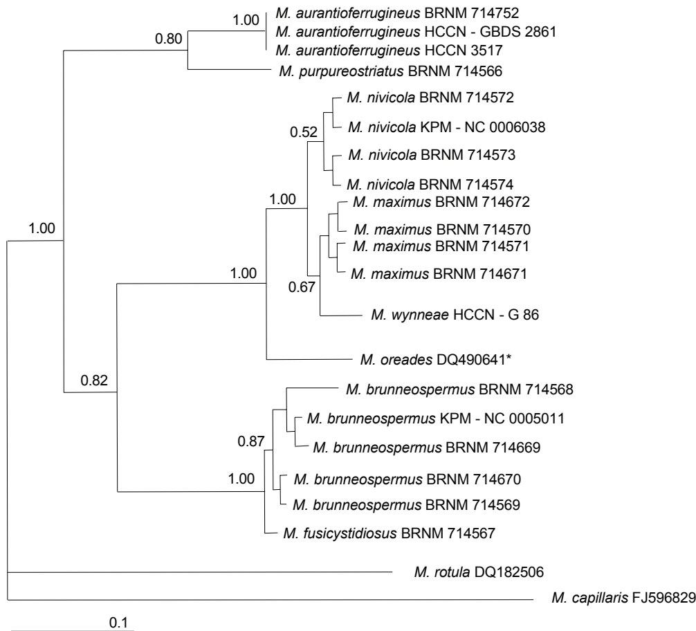
Fig. 10 Phylogenetic tree – ITS. Phylogenetic tree for Marasmius sect. Globulares species inferred from a Bayesian analysis of the complete ITS region (ITS1, 5.8S rDNA, and ITS2), showing mean branch lengths of a 50 % majority rule consensus tree, obtained from an MCMC analysis of one million generations. An asterisk (*) denotes a sequence from GenBank.
