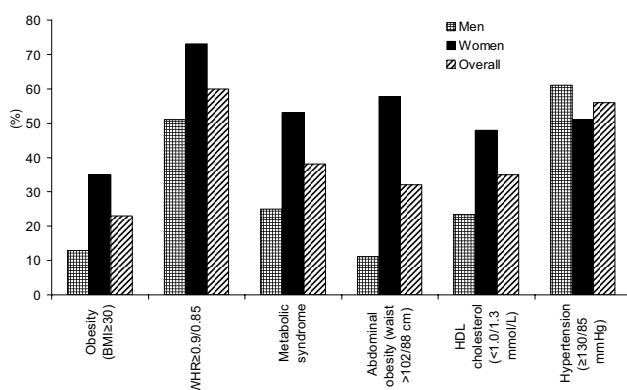
Figure 1 Prevalence of CVD risk factors by gender. (All P-values for gender differences < 0.05 , after adjusting for age).
