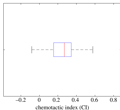
Figure 7. Boxplot of the chemotactic index of 16 simulated cells migrating in an initial saturating linear field of chemoattractant. The mean value \bar{CI} = 0.26 and the standard error of the mean s.e.\bar{CI} = 0.04 .
