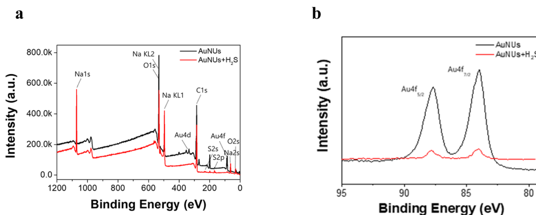
Fig. 2 (a) Wide-scan XPS spectra of AuNUs (black) and AuNUs- \text{H}_2\text{S} (red). (b) XPS Au4f spectra of AuNUs (black) and AuNUs- \text{H}_2\text{S} (red) at pH 4.0 and 25 ^\circ\text{C} in 20 mM NaCl.
