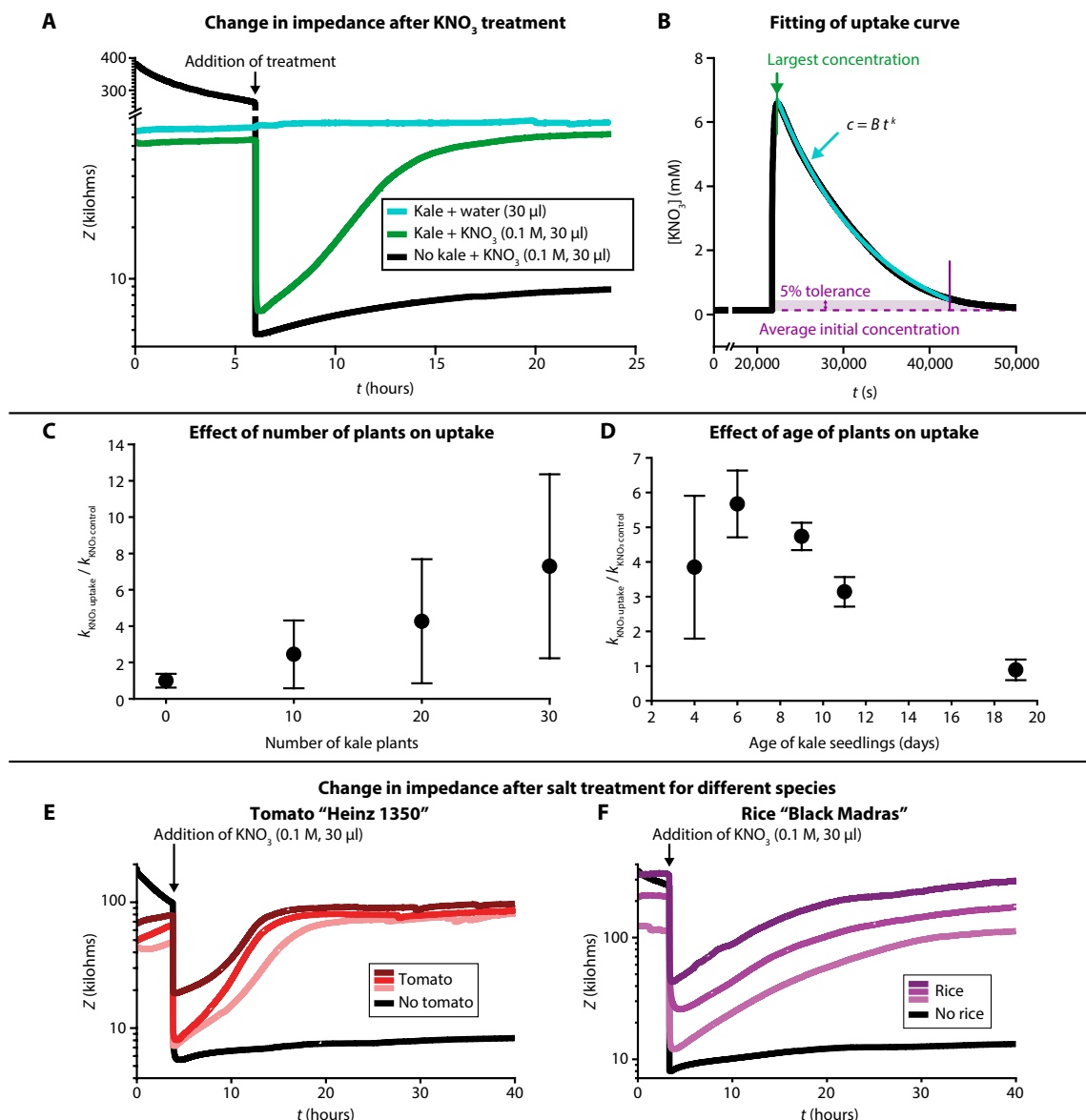
Fig. 4. Uptake of ions by kale, tomato, and rice seedlings. (A) Kale seedlings grown on filter paper were placed onto the impedance sensor within TETRIS, and the electrical impedance was measured in real time. \text{KNO}_3 (0.1 M, 30 \mu\text{l} ) was then added to the filter paper after a rest period of at least 3 hours (arrow). The impedance slowly increased as ions were taken up by the seedlings and the salt concentration in the paper decreased (green signal). This is compared to empty paper substrate (no plants present), where the impedance remained low (black signal), and plants on paper with only water added instead of salt solution, where the impedance remained high (teal signal). Data smoothed in OriginPro using a percentile filter (50th percentile, 100 points of window). (B) An exponential curve of the form c = Bt^k was plotted between the point of largest salt concentration measured up to where the curve meets the initial baseline concentration, with 5% tolerance. k was found and set as the uptake amount. (C) Effect of number of 9-day-old kale seedlings on relative amount of uptake of constituent ions of \text{KNO}_3 . Error bars indicate 1 SD ( n = 3 ). (D) Effect of age of kale (30 plants) on relative amount of uptake of constituent ions of \text{KNO}_3 . Error bars indicate 1 SD ( n = 3 ). Adding salts to different species: (E) \text{KNO}_3 (0.1 M, 30 \mu\text{l} ) added to 20 tomato Heinz 1350 seedlings on paper (red signal) or empty paper substrate (black signal) and (F) \text{KNO}_3 (0.1 M, 30 \mu\text{l} ) added to eight rice Black Madras seedlings on paper (purple signal) or empty paper substrate (black signal). Data smoothed in OriginPro using a percentile filter (50th percentile, 100 points of window).
