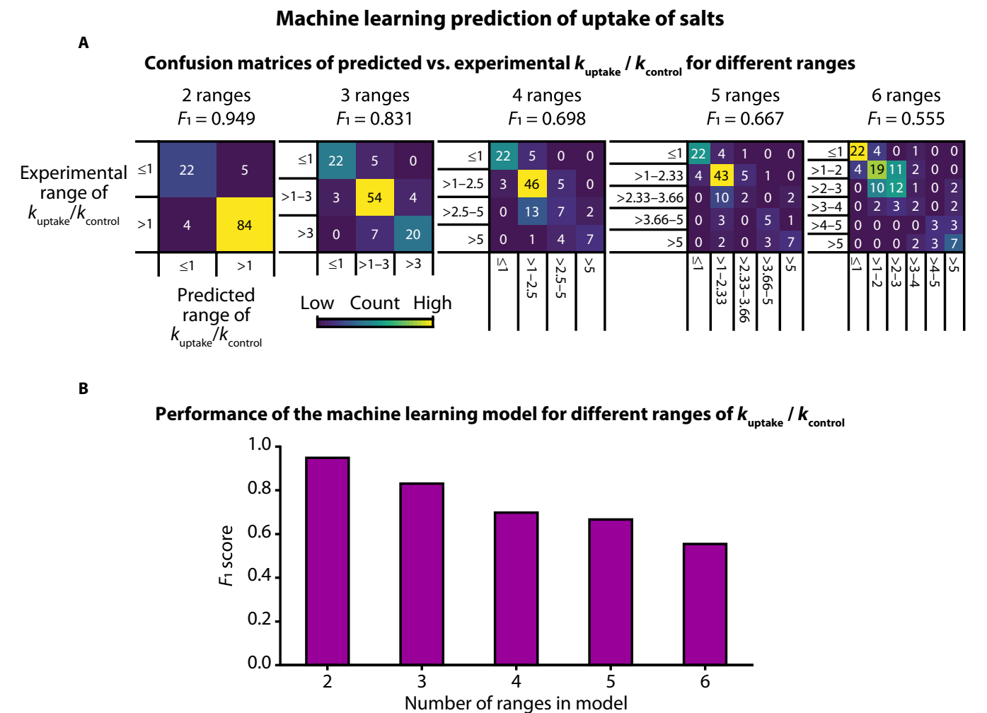
Fig. 6. Using machine learning algorithms to predict normalized rate of uptake ( k_{\text{uptake}}/k_{\text{control}} ). (A) Confusion matrices comparing predicted and experimentally obtained ranges of ( k_{\text{uptake}}/k_{\text{control}} ). (B) F_1 score (a metric of accuracy combining precision and recall) decreases with increasing number of ranges in the machine learning model.
