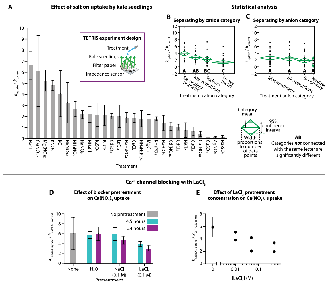
Fig. 5. Effect of different salts on normalized rate of uptake. (A) Rate of uptake of salt from paper disc with 30 kale seedlings (9 days old), relative to control without plants, using TETRIS. (Values at or below 1 are considered to have a net zero or negative ion uptake.) Error bars indicate 1 SD [CdCl 2 , KCl, and NaCl: n = 3; CaCl 2 and Ca(NO 3 ) 2 : n = 6; LaCl 3 : n = 7; all others: n = 4]. Statistical analysis showed significant differences between some cation classes (B), but not between anion classes (C), where confidence diamonds show mean uptake, 95% confidence interval and number of data points, and letters show categories with or without significant difference. (D) Pretreatment of 30 kale seedlings (9 days old) with deionized water, NaCl (0.1 M), or LaCl 3 (0.1 M) for 4.5 or 24 hours and their effect on the relative change in concentration of Ca(NO 3 ) 2 . Error bars indicate 1 SD (none: n = 6; LaCl 3 24 hours: n = 4; all others: n = 3). (E) Pretreatment of 30 kale seedlings (9 days old) with varying concentrations of LaCl 3 for 4 hours and the effect on the relative change in concentration of Ca(NO 3 ) 2 . Error bars indicate 1 SD ( n = 2).
