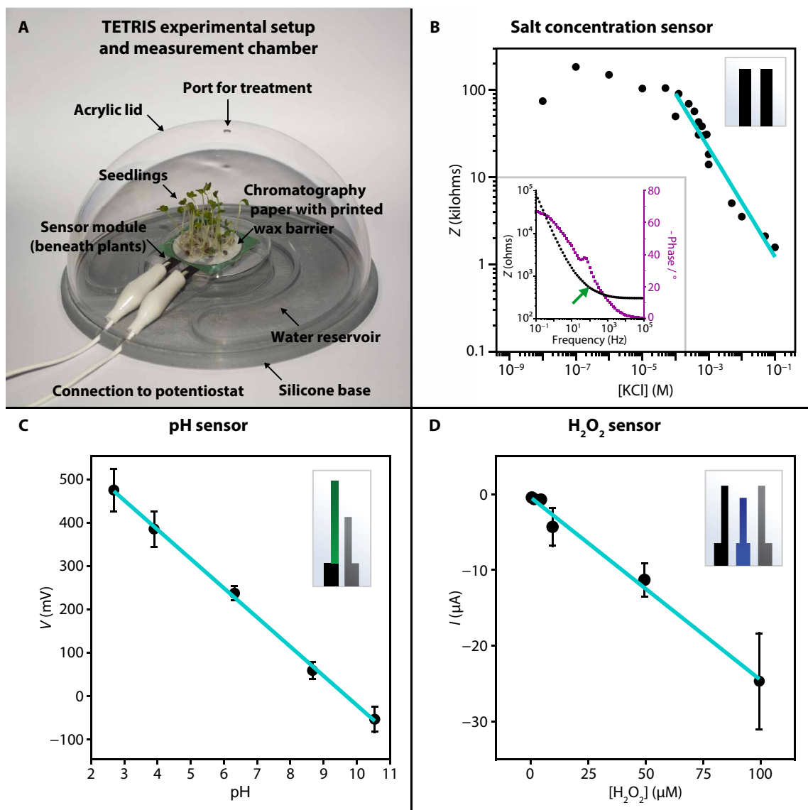
Fig. 2. Characterization of TETRIS. (A) Photograph of TETRIS, where single or multiple sensors can be placed under seedlings grown on paper (kale seedlings pictured). (B) Average impedance response of our salt concentration sensor to various concentrations of KCl at 2 kHz. Solid teal line indicates linear fit of linear range of data. Inset shows the Bode plot of electrochemical impedance spectrum in 0.1 M KCl, where the green arrow shows our chosen frequency of 2 kHz. (C) Calibration curve of pH sensor in 1 M KCl. Error bars show 1 SD ( n = 8 ). (D) Calibration curve of the H_2O_2 sensor in 1 M KCl. Error bars show 1 SD (100 \mu M : n = 4 ; 2 \mu M : n = 2 ; 5 to 50 \mu M : n = 3 ). Sensor design displayed in the top right corner of each plot (B to D).
