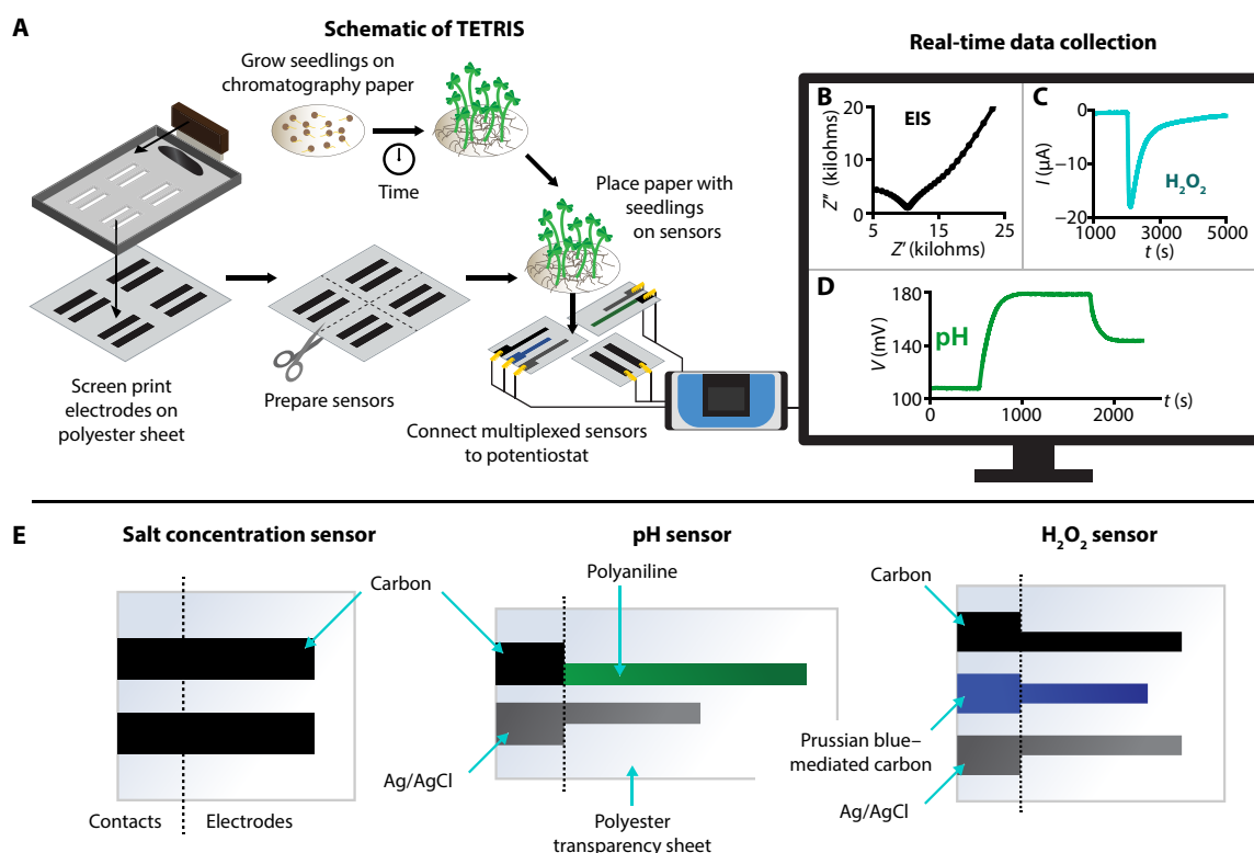
Fig. 1. Setup of TETRIS. (A) Schematic of TETRIS, showing sensor fabrication, growth of seedlings, and recording of measurements using a standard laboratory potentiostat. (B) Electrochemical impedance spectroscopy Nyquist plot of a paper disc with 30 kale seedlings (9 days old). (C) \text{H}_2\text{O}_2 sensing during the addition of \text{H}_2\text{O}_2 (1 mM, 20 \mu\text{l} ) to a paper disc with KCl (1 M, 180 \mu\text{l} ). (D) pH sensing during the addition of \text{H}_2\text{SO}_4 and NaOH to deionized water. (E) Design and materials of our salt concentration, pH, and \text{H}_2\text{O}_2 sensors; illustrations not to scale.
