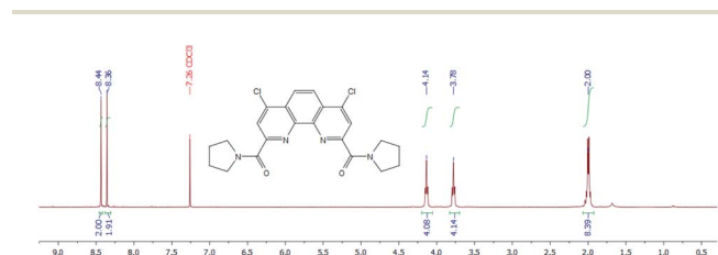
Fig. 9 1 H NMR spectrum of 3a in CDCl 3 at 25 °C.
