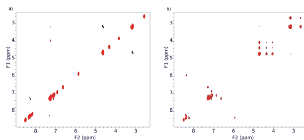
Fig. 11 ROESY 1 H NMR spectra of 3f in CDCl 3 at -30 °C (a) and 25 °C (b).
