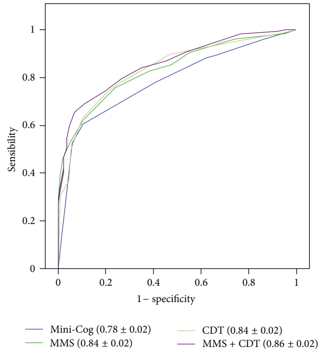
FIGURE 2: ROC curves for detection of CI (MCI or dementia). The area ( \pm SD) under the receiver operating characteristic curve (ROC) is indicated. MMS: Mini-Mental State; CDT: Clock Drawing Test; CI: cognitive impairment; MCI: mild cognitive impairment.
