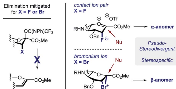
Scheme 8 Pseudo-stereodivergent sialylation.
