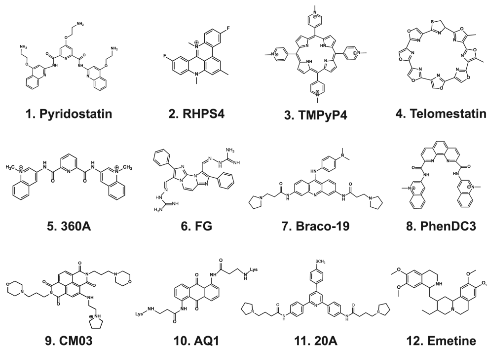
Figure 2. Chemical structures of G4 binders.
