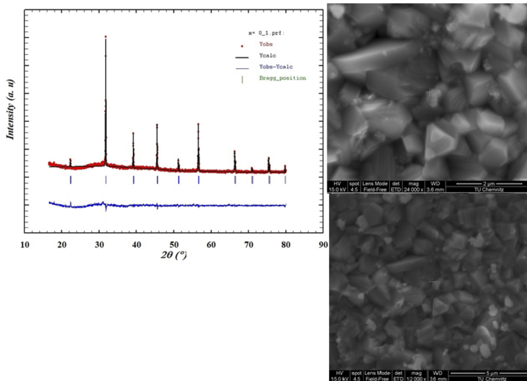
Fig. 1 XRD pattern for the tetragonal ceramic 0.8(\text{Ba}_{0.8}\text{Sr}_{0.2})\text{TiO}_3 - 0.2(\text{Bi}_{0.85}\text{Yb}_{0.15})\text{FeO}_3 at room temperature and SEM micrographs of the ceramic surface.
