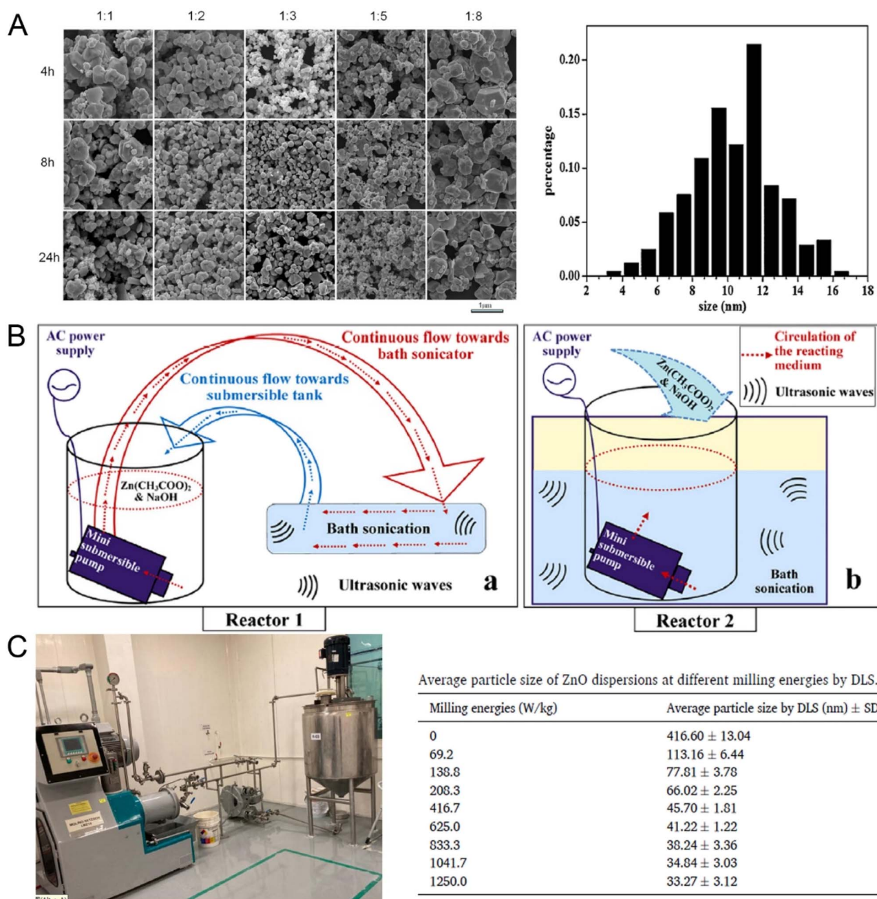
Fig. 9 Large-scale production of NPs. (A) Left panel, FESEM images of Ag NPs. The columns present samples produced from different molar ratios of \text{AgNO}_3 to AA, and the rows show materials obtained at different reaction times. Right panel, the size distribution of AgNPs produced by \text{AgNO}_3 and AA with a molar ratio of 1 : 3 after 4 h. Reproduced from ref. 349 with permission from Elsevier, copyright 2015. (B) Schematic representation of the working of the MSP-assisted sonochemical flow loop reactor (a), and MSP-assisted sonochemical mixing reactor (b). ZnO-NPs and ZnO-NLs are the products from reactors 1 and 2 respectively. Reproduced from ref. 363 with permission from Elsevier, copyright 2019. (C) Left panel, milling mechanism composed of a high-energy ball mill and a dispersion tank for large-scale production of ZnO NPs. Right panel, the average particle size of ZnO dispersions at different milling energies by DLS. Reproduced from ref. 365 with permission from Elsevier, copyright 2023.
