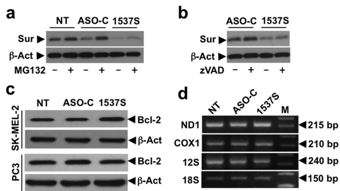
FIGURE 8. Down-regulation of survivin ( Sur ) is not affected by proteasome or caspase degradation. a , SK-MEL-2 cells were treated as described in the presence or absence of 5 \mu M proteasome inhibitor MG132, added 4 h before transfection. Western blot at 24 h post-transfection shows that the inhibitor did not revert the decrease in survivin. \beta -Actin, \beta -actin. b , the same as in a , but transfection was carried out in the presence or absence of 40 \mu M z-VAD-fmk for 24 h. The presence of z-VAD-fmk did not significantly revert the reduction in survivin elicited by transfection with ASO-1537S. c , ASK does not affect the expression of Bcl-2. SK-MEL-2 and PC3 cells were seeded and transfected as in a for 24 h and analyzed by Western blot, revealing that Bcl-2 expression was not affected by ASO-1537S. d , ASK does not affect mitochondrial transcription. SK-MEL-2 cells were transfected for 24 h as described before. Total RNA was isolated and subjected to RT-PCR amplification for 25 cycles (ND1 and COX1) or 20 cycles (12S) and using 18S rRNA (15 cycles) as control. No change in the expression of ND1, COX1, and 12S mitochondrial RNA was observed. M , 100-bp ladder.
