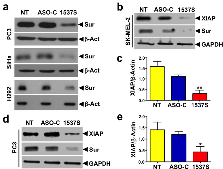
FIGURE 7. ASK induces down-regulation of survivin ( Sur ) and XIAP in other tumor cell lines. a , PC3, SiHa, and H292 cells were transfected according to the conditions described in Table 1, with ASO-C or ASO-1537S or left untreated ( NT ), and cell lysates were analyzed by Western blot. Transfection with ASO-1537S also induces down-regulation of survivin in these cells, as compared with controls. \beta -Actin, \beta -actin. b , ASK induces down-regulation of XIAP. SK-MEL-2 cells were transfected as described before for 24 h and analyzed by Western blot with anti-XIAP and anti-survivin antibody using GAPDH as loading controls. XIAP and survivin are reduced by ASK, compared with controls. c , this result was confirmed in three different experiments (**, p < 0.01 ). d and e , the same result was obtained with PC3 cells (*, p < 0.05 ).
