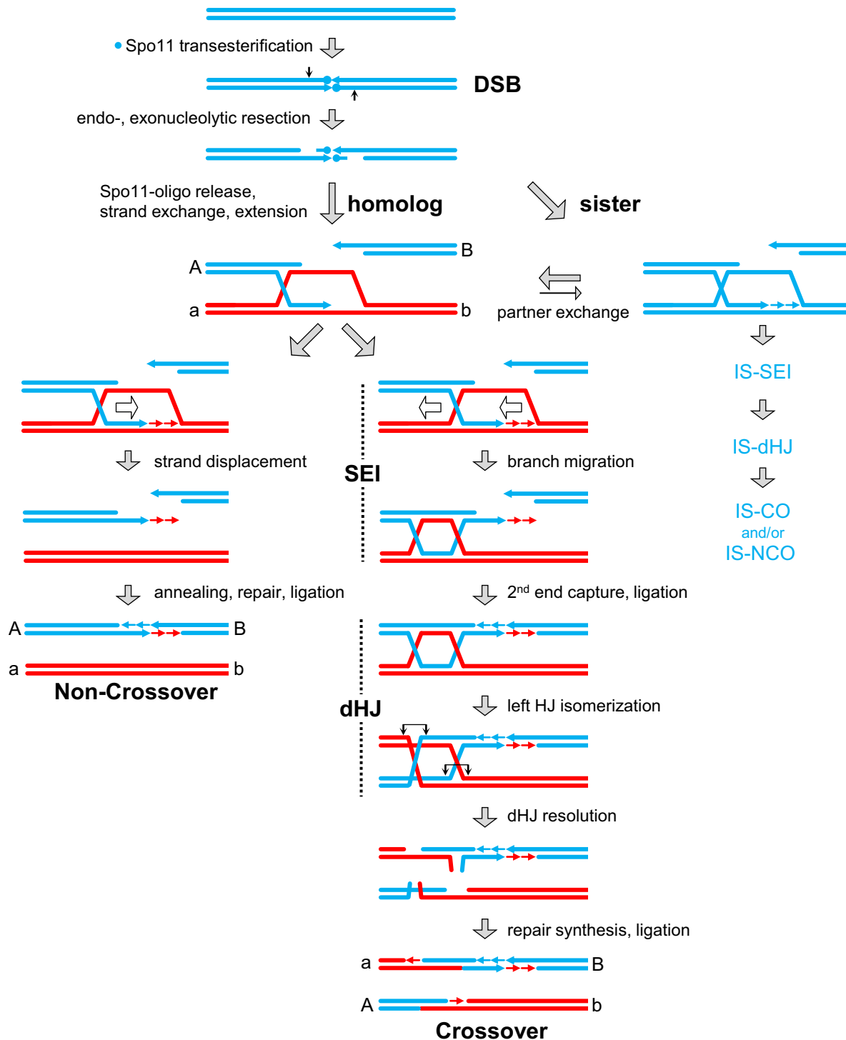
Fig. 4. Homologous recombination pathways during meiosis. The recombination model shows two allelic double stranded DNA molecules from homologous chromosomes in blue and red. Spo11, covalently attached to the 5' ends of the cleaved strand, is indicated by a filled circle. 3' ends and newly synthesized DNA are indicated by arrowheads and short arrows in blue or red, respectively, without consideration of ligation status. Recombination between sister chromatids likely involves equivalent intermediates as recombination between homologs, and only the names of the relevant molecules are provided (intersister single end invasion, IS-SEI; intersister double Holliday junction, IS-dHJ). Single end invasion (SEI) and double Holliday junction (dHJ), molecules are thought to exist in two conformations, as indicated by the dotted vertical line in black. Movements of Holliday junctions are indicated by open arrows. To generate crossovers from dHJs, the two tandem Holliday junctions need to be resolved with opposite directionalities, either by two single stranded nicks that flank each junction or via nicks of both crossing strands (see text for details).
