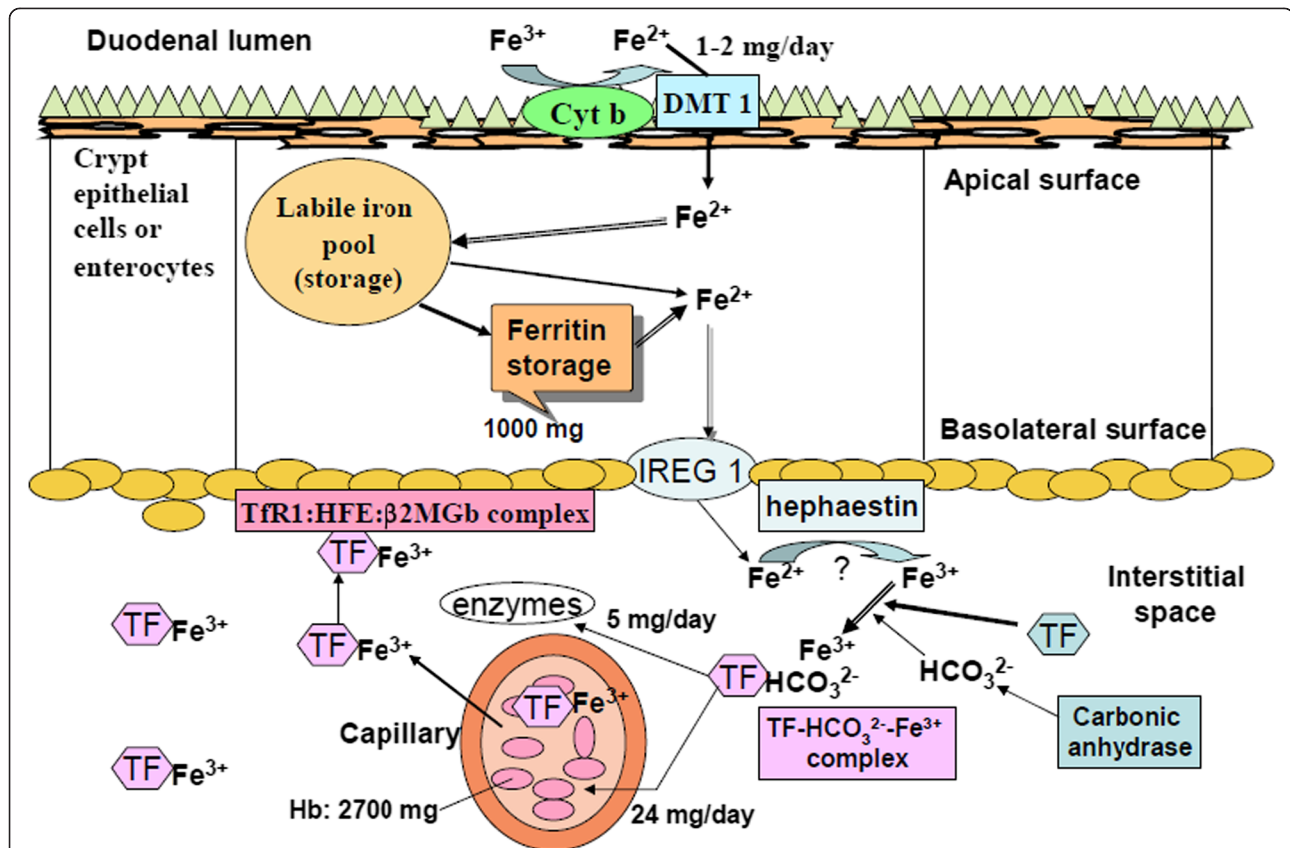
Figure 5 The highly elevated serum transferrin due to lack of effective formation of ferric ion-carbonate-transferrin complex. The dissociation constant of this complex is K_d = 10^{-22} [15]. Iron is absorbed from the duodenal lumen t by divalent-metal transporter 1 (DMT1) after reduced by the cytochrome b, Cyt-b. Intracellular iron enters the labile iron pool (LIP), either exported by iron-regulated protein 1 (IREG1) and then oxidized by hephaestin or, stored in ferritin cores [14] up to 1000 mg Fe. In the presence of bicarbonate ions supplied from anhydrase I, transferrin (Tf) and Fe 3+ ions form a ternary complex 'transferrin-bicarbonate-ferric ion complex' to facilitate transport of ferric ions to be incorporated into hemoglobin [16,17]. A complex of transferrin receptor 1 (TfR1), the hemochromatosis protein (HFE) and β2-microglobulin, is supposed to act as primarily the iron-biosensor [14].
