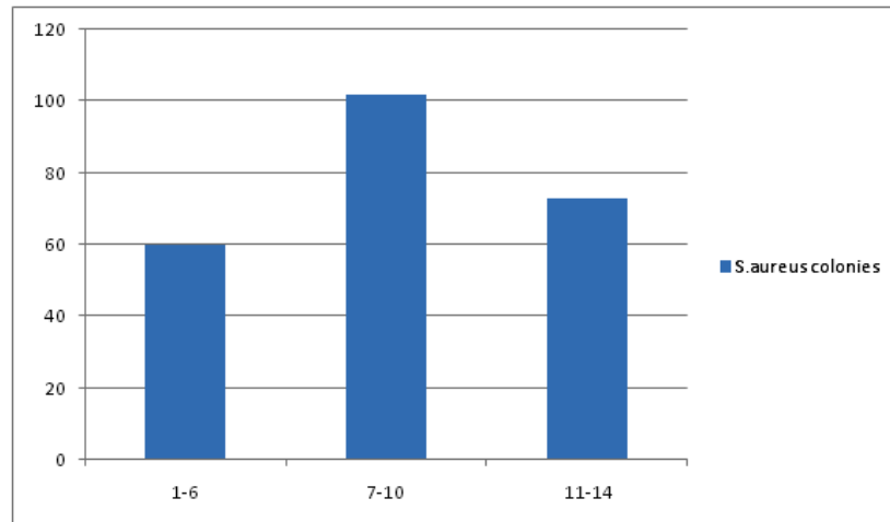
Fig. 1. Frequency of S. aureus colonized subjects in each age group
