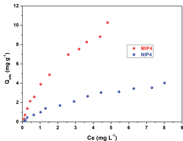
Fig. 7 Adsorption isotherms of MIP4 and NIP4. Adsorption condition: 10 mg of polymer, pH: 6.7, adsorption solution: 0.12\text{--}10.10 \text{ mg L}^{-1} CIP in deionized water, temperature 30 \pm 0.5 °C, shaking time: 3 h.
