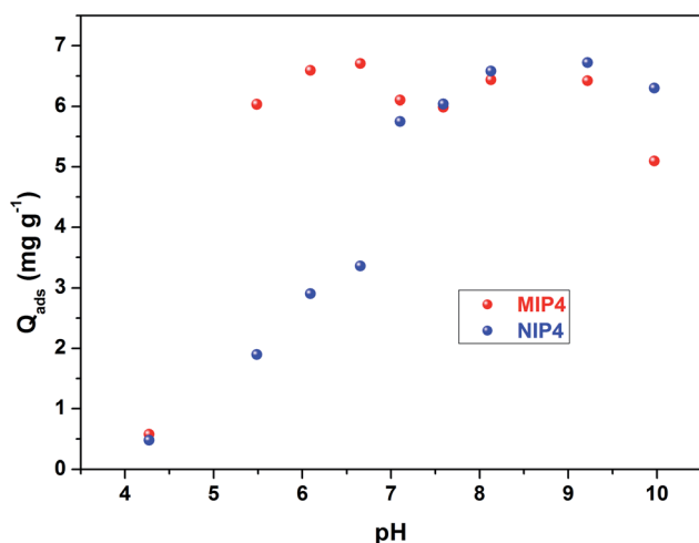
Fig. 6 Effect of pH on the adsorption properties of MIP4 and NIP4. Adsorption condition: 10 mg of polymer, pH: 4–10, adsorption solution: 20 mL of 5 \text{ mg L}^{-1} CIP in deionized water, temperature: 30 \pm 0.5 °C, shaking time: 3 h.
