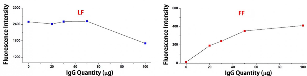
Fig. 3 Comparison of lectin-first and fluorescence-first quantification of glycoproteins. (A) Lectin-first (LF): glycoproteins bind to lectins, removing non-targeted glycoproteins/proteins. Lectin-bound glycoproteins are labeled with a fluorescent reagent (AF488), and excess reagents are washed away. The labeled glycoproteins are quantified by a fluorescent detector. (B) Fluorescence-first (FF): glycoproteins/proteins are labelled with a fluorescent reagent (AF488), and excess reagents are quenched and removed by ultrafiltration. The labeled glycoproteins are specifically enriched by lectin affinity, and other components are removed, followed by fluorescence quantification. (C) Quantification of IgG using LF (left) and FF (right), where LF quantification showed no linear relationship between fluorescence intensity and IgG quantity due to concomitant lectin labeling. Conversely, FF quantification showed that the amount of IgG was proportional to the fluorescence intensity, indicating that lectin affinity was not affected by fluorescent labeling of glycoproteins.
