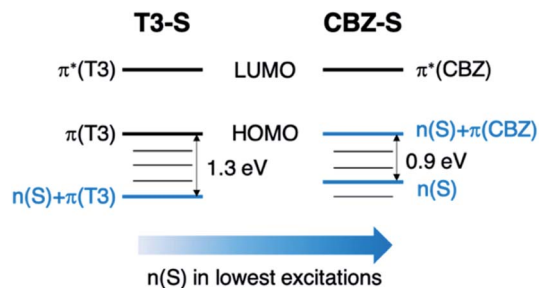
Fig. 9 Schematic comparison of frontier orbitals in terthiophene (T3-S) and carbazole (CBZ-S) sulfide-bridged chromophores.
