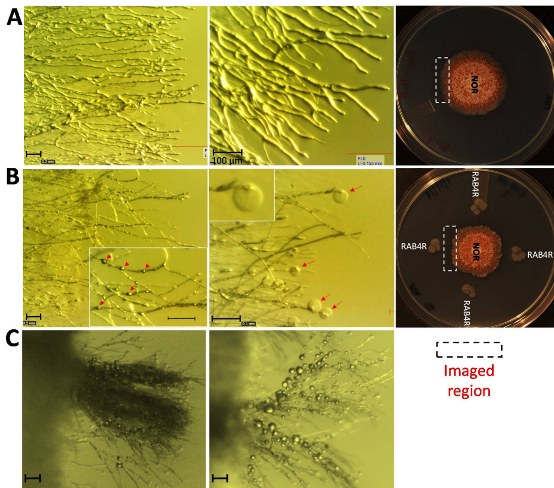
Figure 5. RAB4R induces intercalary cell swelling, tip lysis, abnormal branching, and increased surface hydrophobicity in A. flavus . (A) The edge of A. flavus colony at 30 \times (left panel) and 63 \times (right panel) magnification showing uniformly-growing well-rounded hyphal tips. (B) The edge of A. flavus colony from the growth inhibition zone induced by RAB4R at 30 \times magnification, showing an irregular growing edge with hyphae showing cell swelling (left panel). The inset show 63 \times magnification to highlight swollen cells marked by arrow heads. The right panel shows hyphal tip lysis marked by red arrows. The inset show 63 \times magnification to highlight a lysed hyphal tip. (C) Abnormal hyphal branching and increased hydrophobicity are indicated by accumulation of water droplets on the hyphal surface in the inhibition zone. The scale bar in each panel is equal to 100 \mu m.
