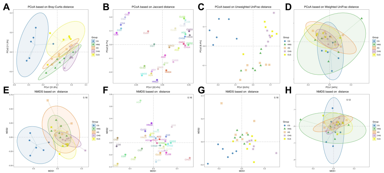
Figure 5 The \beta -diversity of gut microbiota based on NMDS analysis. (A) PCoA based on Bray-Curtis distance. (B) PCoA is based on Jaccard distance. (C) PCoA based on Unweighted UniFrac distance. (D) PCoA based on Weighted UniFrac distance. (E) NMDS based on Bray-Curtis distance. (F) NMDS based on Jaccard distance. (G) NMDS based on Unweighted UniFrac. (H) NMDS based on Weighted UniFrac.
