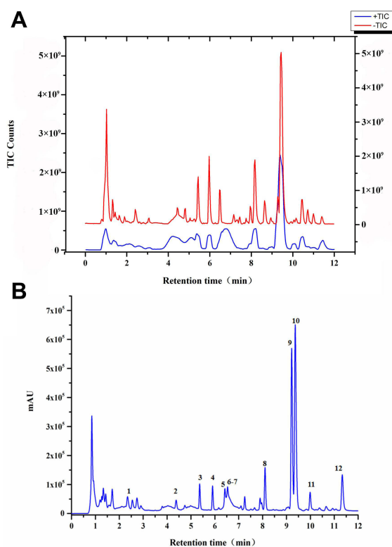
Figure 1 Main chemical constituents of CILF (A) UPLC-Q/Orbitrap HRMS total ion chromatogram of CILF. (B) UPLC chromatogram of CILF at a wavelength of 254 nm. 1, Shanzhiside; 2, Inopyranosid; 3, Chlorogenic acid; 4, Cryptochlorogenic acid; 5, Isochlorogenic Acid B; 6, Isochlorogenic acid A; 7, Isochlorogenic acid C; 8, Genipin l-gentiobioside; 9, Puerarin; 10, Capparoside A; 11, Puerarin 6''-O-xyloside; 12, Daidzin.
