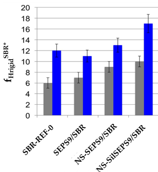
Figure 5. Fraction of rigid rubber ( f_{\text{Hrigid}}^{\text{SBR}^*} , %) determined for the uncured (grey) and vulcanized (blue) samples from the analysis of ^1\text{H} FID's, as described in the text.
