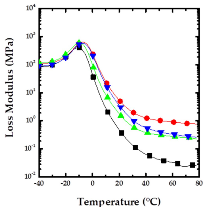
Figure 2. Loss modulus ( E'' ) vs. temperature for V-SBR-REF-0 ( \blacksquare —black line), V-SepS9/SBR ( \bullet —red line), V-NS-SepS9/SBR ( \blacktriangle —green line), and V-NS-SilSepS9/SBR ( \blacktriangledown —blue line).
