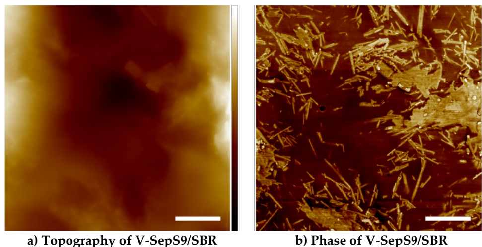
Figure 7. Tapping-Mode (TM) topographic (a) and phase (b) images of V-SepS9/SBR PNC. The white scale bar is 1.0 \mu\text{m} . The Z-range is 1.0 \mu\text{m} and the phase scale is 25 degrees.
