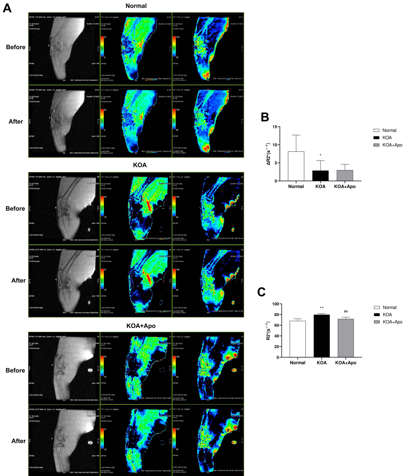
Figure 2 Acupuncture relieved the state of hypoxia. (A) Representative T2* images and pseudo-color T2* images and pseudo-color R2* images in each group. And ROIs used to delineate the synovium to derive reactivity maps of normoxia and hyperoxia (using a mixture of 95% oxygen (O 2 ) and 5% carbogen (CO 2 ) for hyperoxia stimulus). (B) ΔR2* changes between groups. *P < 0.05 vs the Normal group. (C) R2* changes between groups. **P < 0.01 vs the Normal group. ##P < 0.01 vs the KOA group.
