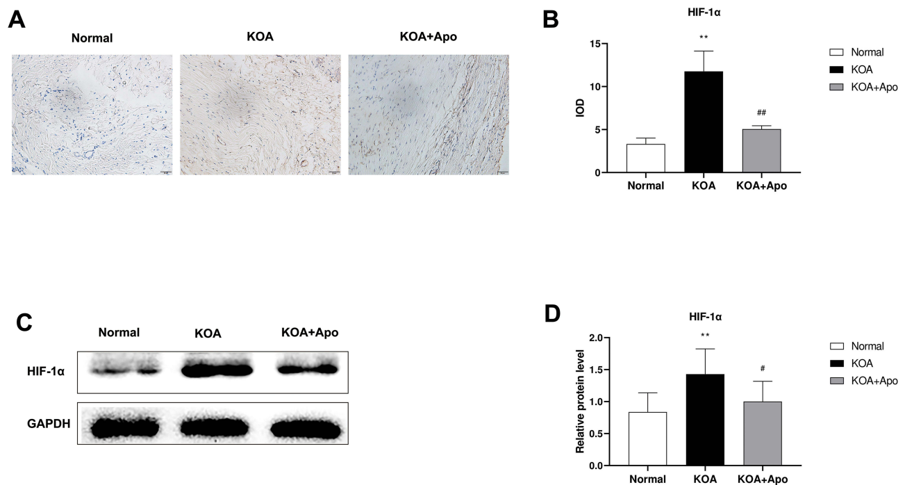
Figure 3 Acupuncture reduced the expression of HIF-1 \alpha in rabbit synovial tissue. (A) Representative HIF-1 \alpha IHC sections of synovial tissues in each group, 200 \times . (B) Relative IOD value in each group. Semiquantification of IHC sections was evaluated by calculating the positive areas of HIF-1 \alpha . Data were analyzed by Image J Pro Plus 6.0. ** P < 0.01 vs the Normal group. ### P < 0.01 vs the KOA group. (C) Typical protein bands of HIF-1 \alpha . (D) Protein level comparison of HIF-1 \alpha between groups. ** P < 0.01 vs the Normal group. # P < 0.05 vs the KOA group. Data were analyzed by Image J.
