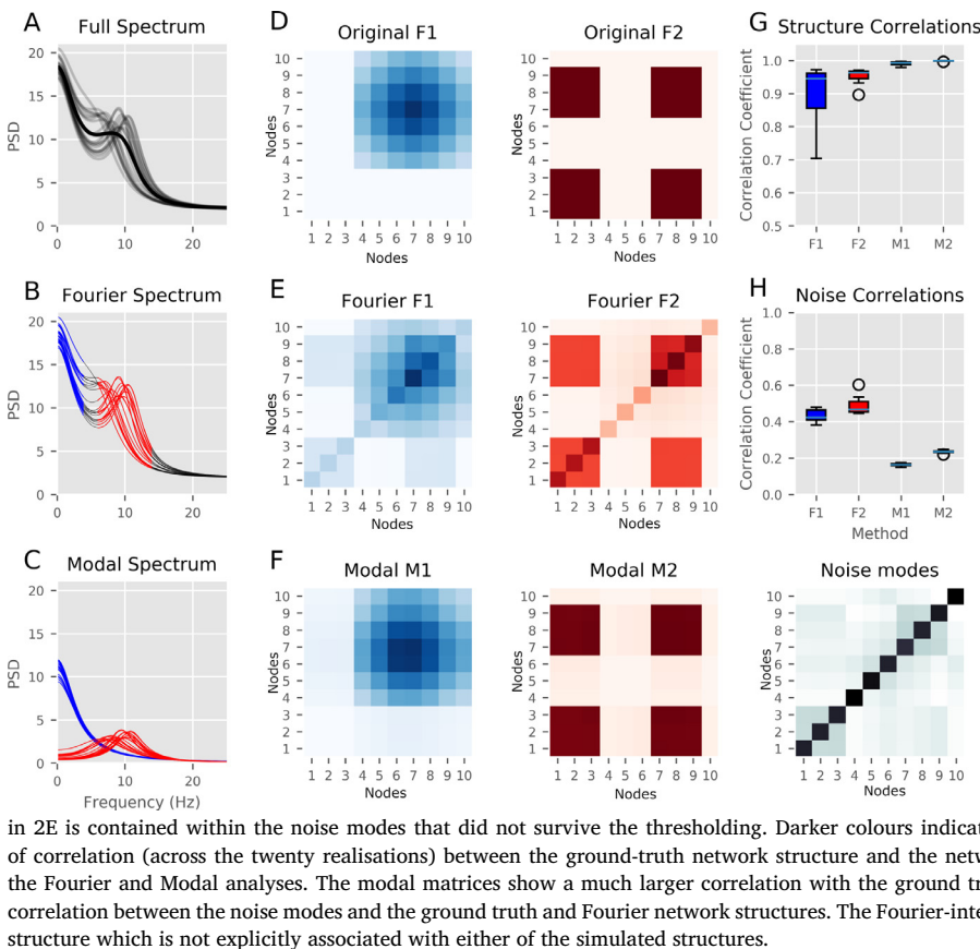
Fig. 2. Power spectra and networks from the group simulation. A: The PSD of node 7 for all 20 realisations with variable spectra (gray) and the group average (black). B: Fourier-based PSD of node 7. The PSDs are split into pre-specified ‘low’ and ‘high’ frequency bands (in blue and red respectively). Though these capture the features around each frequency, they do not account for either individual variance in peak frequency or overlap between adjacent frequencies. C: Modal-based PSD of node 7. The modal spectra identified by thresholding the damping times of each mode of the modal decomposition and assigning each mode to its closest band (low in blue or high in red). The modal spectrum contains a single peak per mode and allows for variability in peak frequency between participants. D: Original network structure matrices. This figure shows the ground truth for the simulations generated in Fig. 1. Darker colours indicate higher power in each node or connection. E: Fourier-based network structure reconstruction. The network structure estimated from the Fourier-integration approach based on the bands in 2B, this captures the main structure with some interference from the adjacent frequency band. Darker colours indicate higher power in each node or connection. F: Modal-based network structure reconstruction. The network structure estimated from the modal bands seen in 2C. Here, the two spectrally distinct networks are properly resolved and there is little interference between the two. The diagonal structure in 2E is contained within the noise modes that did not survive the thresholding. Darker colours indicate higher power in each node or connection. G: The level of correlation (across the twenty realisations) between the ground-truth network structure and the network structure extracted for each individual run and both the Fourier and Modal analyses. The modal matrices show a much larger correlation with the ground truth than the Fourier-integration derived matrices. H: The correlation between the noise modes and the ground truth and Fourier network structures. The Fourier-integration matrices have a large correlation with the diagonal structure which is not explicitly associated with either of the simulated structures.
