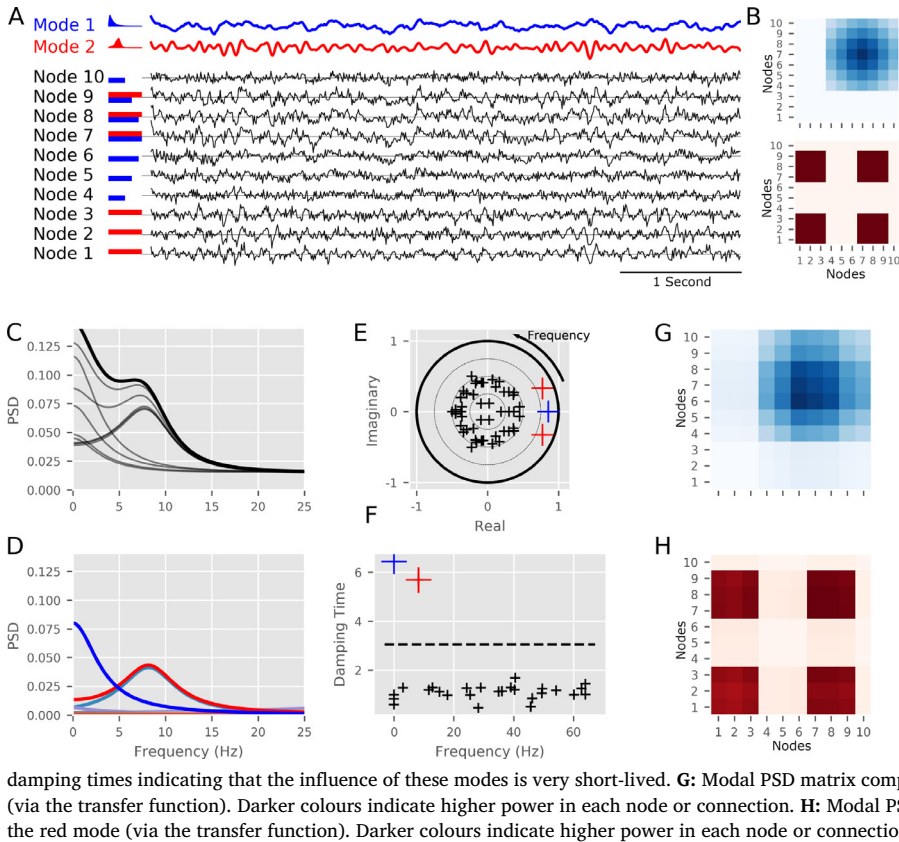
Fig. 1. The simulations and modal decomposition for a single realisation of the simulated data. A: Summary of the simulation. ten nodes are generated from linear combinations of two modes with different spectra. The modes are shown in blue and red with the nodes in black, horizontal bars indicate the weighting of the two modes into each of the 10 nodes. B: Summary of the true network structure of the two modes. Darker colours indicate higher power in each node or connection. C: The power spectral density from ten nodes. These capture the gradual drop in frequency from 0Hz and a peak around 9Hz split across the different nodes. D: The modal power spectrum for the node highlighted in black in C. The gradual slope from 0Hz and the 9Hz peak are clearly isolated as distinct resonances. The remaining modes have very low amplitudes with no clear peaks. E: z-plane representation of the modal eigenvalues (shown as crosses). The frequency of each mode relates to its angle as it increases counter-clockwise from (1,0) to (-1,0). Negative frequencies correspond to angles increasing clockwise from (1,0) to (-1,0). The two high-power modes from D are clearly visible as the modes with the largest magnitude (red and blue). The remaining modes have small magnitudes and have evenly distributed angles (black crosses). F: Damping-time of each mode as a function of frequency. The red and blue modes have significantly longer damping times than the null distribution (99% threshold shown as the dotted line). These relate to 0Hz and 9Hz resonances in the data. The remaining modes have short damping times indicating that the influence of these modes is very short-lived. G: Modal PSD matrix computed from the eigenvectors associated with the blue mode (via the transfer function). Darker colours indicate higher power in each node or connection. H: Modal PSD matrix computed from the eigenvectors associated with the red mode (via the transfer function). Darker colours indicate higher power in each node or connection.
