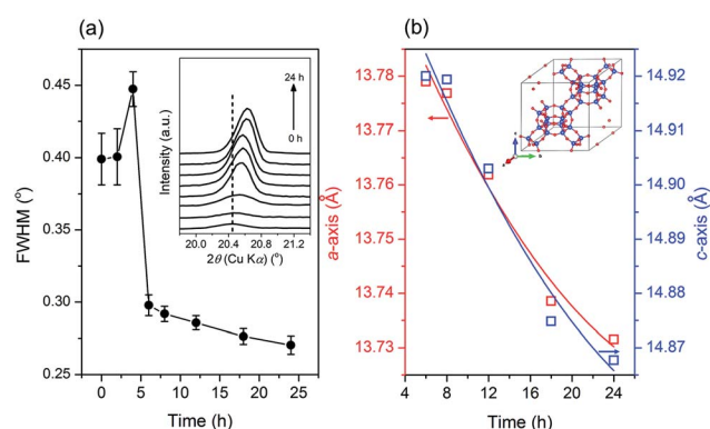
Fig. 4 (a) FWHM of the (20 \bar{1} ) plane reflection and (b) lattice parameters of the products obtained after different periods of hydrothermal treatment of initial mixtures with the following molar composition, 1SiO 2 : 0.05Al 2 O 3 : 0.3Na 2 O : 0.1K 2 O : 100H 2 O, at 170 °C.
