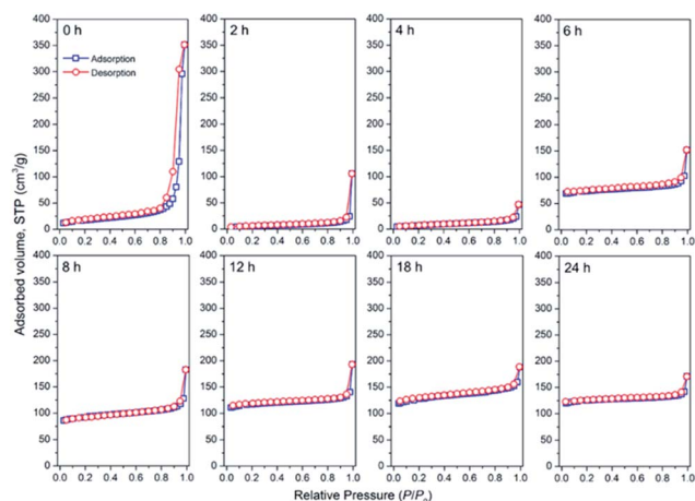
Fig. 10 \text{N}_2 adsorption–desorption isotherms of the products obtained after different periods of hydrothermal treatment of initial mixtures with the following molar composition, 1\text{SiO}_2 : 0.05\text{Al}_2\text{O}_3 : 0.3\text{Na}_2\text{O} : 0.1\text{K}_2\text{O} : 100\text{H}_2\text{O} , at 170 \text{ }^\circ\text{C} in the presence of CHA seeds (10 wt% of the total silica).
