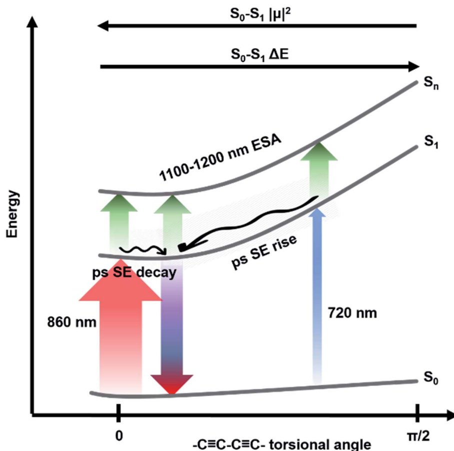
Fig. 4 Level diagram representing ground and excited states and fast dynamics of c-Pn por . Transitions observed via fsTA after excitation with ultrashort 720 nm (blue upward arrow) or 860 nm (red upward arrow) pump pulses. Stimulated emission from the minimum of the excited state potential energy surface is represented as a blue/red downward arrow. S_1 \rightarrow S_n NIR excited state absorption is represented as green upward arrows. The arrows thickness is proportional to the transition dipole moment of each transition. Relaxations in the excited state potential energy surface are represented by wavy arrows. Assignments are reported as well.
