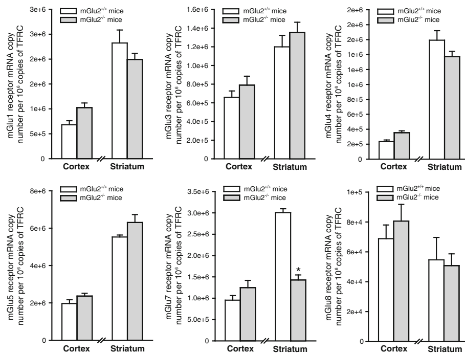
Fig. 4 Analysis of mGlu receptor subtypes in the cerebral cortex and striatum of mGlu2 +/+ and mGlu2 -/- mice. Quantitative PCR analysis of mGlu1, mGlu3, mGlu4, mGlu5, mGlu7 and mGlu8 receptors mRNA levels in mGlu2 +/+ and mGlu2 -/- mice. mRNA values, expressed as copy number, were normalized to TFRC (transferrin receptor protein-1) and are means + S.E.M. of 4–8 mice per group. * p < 0.05 (Student's t test; t_{10} = 4.59 )
