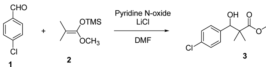
Scheme 1 Synthesis of methyl-3-(4-chlorophenyl)-3-hydroxy-2,2-dimethylpropanoate ( 3 ).
