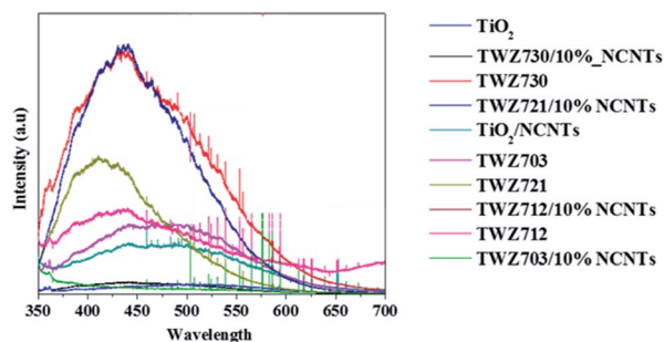
Fig. 8 Photoluminescence emission spectra of TiO 2 , QMМО, and composites.
