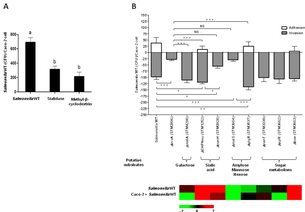
Figure 1. Modulation of carbohydrate-degrading enzymes alter access during invasion of Salmonella WT.
