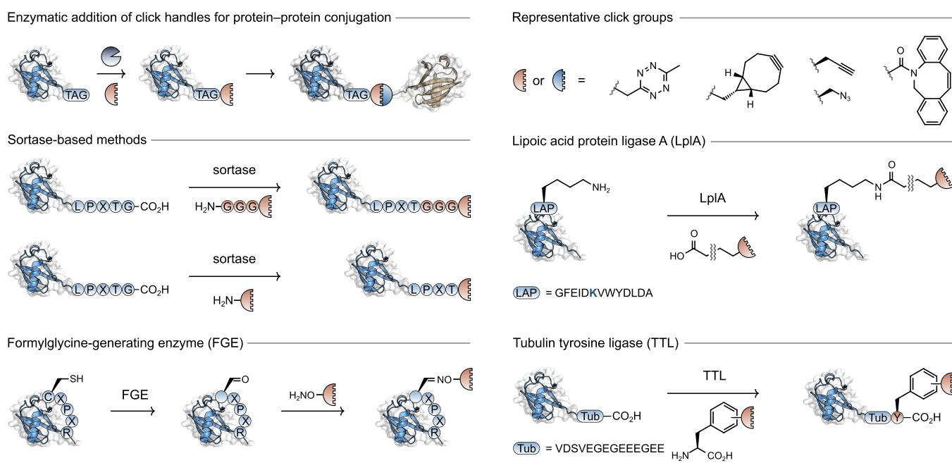
Figure 11. Enzymatic approaches to install click chemistry functional groups for protein–protein conjugation.
