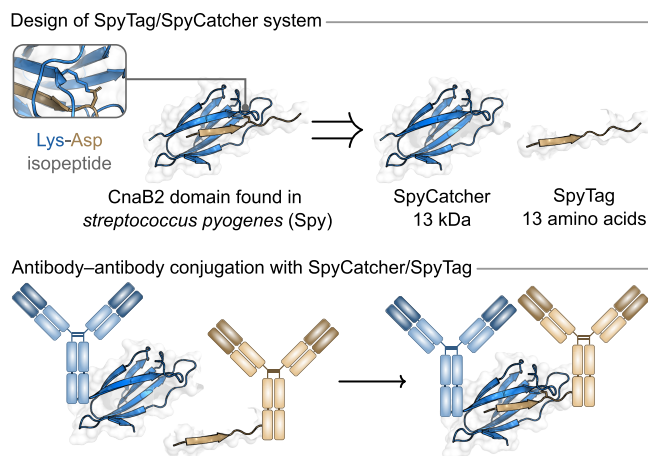
Figure 12. Design of SpyCatcher/SpyTag system and application to preparation of bispecific antibodies.
