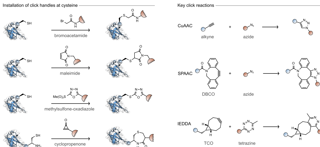
Figure 4. Production of protein–protein conjugates by installing click groups on single cysteine residues.
