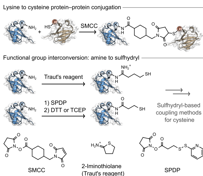
Figure 7. Methods for preparing protein–protein conjugates using lysine conjugation. DTT: Dithiothreitol. TCEP: tris(2-carboxyethyl)-phosphine.
