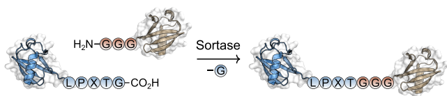
Figure 9. Sortase-based approach for preparing protein–protein conjugates.
