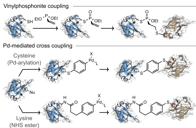
Figure 6. Use of vinylphosphonite and Pd-protein OAC heterobifunctional reagents for sequential protein conjugation through cysteine residues.
