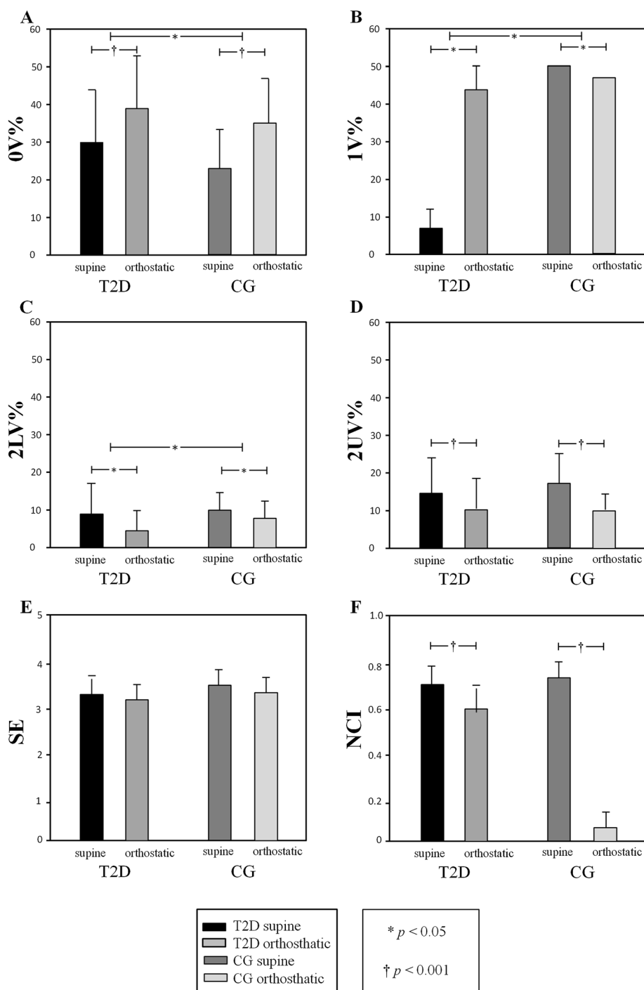
Figure 1 Symbolic dynamics of HRV for individuals with type 2 diabetes (T2D) and and control group (CG). The symbol * indicates p < 0.05 and † indicates p < 0.001 . A: 0V% index; B: 1V% index; C: 2LV% index; D: 2UV% index; E: SE = Shannon entropy; F: NCI = normalized complexity index.
