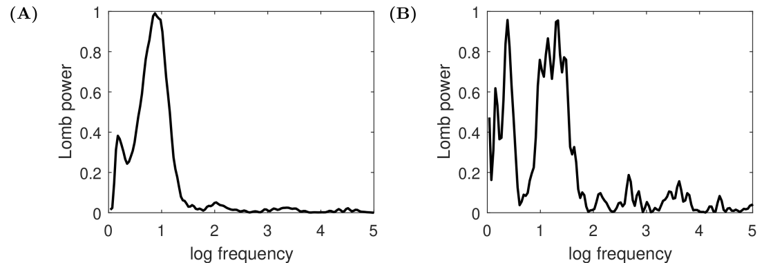
Fig 7. Lomb-periodograms for the trajectories presented in Fig 6. The selection of t_c is done through scanning different possible values between the maximum of the timeseries until the end of sample and then by picking the one giving the highest peak in the Lomb-periodogram. (A) The optimised t_c = 3.46 , which is in the middle of the deflating bubble, (B) the optimised t_c = 13.26 , which is at the top of the bubble. In the second case the sample was shortened so it begins at time 11.5, when the bubble starts to develop.
