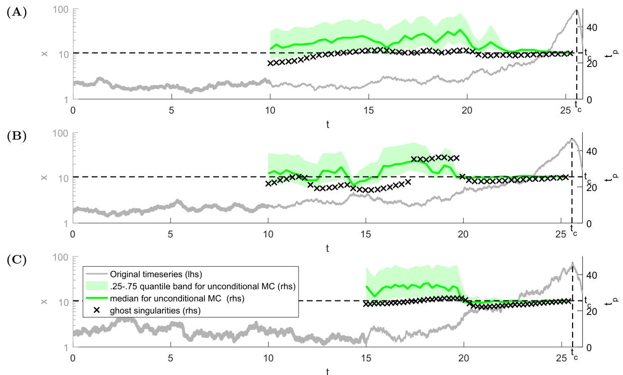
Fig 11. Test of the methodology using the ghosts of finite-time singularities in comparison with Monte Carlo forecasting method. (A) and (B) correspond to two different realizations of the price process for \sigma_x = 0.2 and \sigma_z = 0.01 , (C) corresponds to one realisation generated with \sigma_x = 0.4 and \sigma_z = 0.01 . The stochastic price trajectory is plotted (grey line) with its scale given on the left hand side vertical axis. The scale of the crash time predictions is given by the right hand side vertical axis. The symbols 'x' stand for the predicted time t_p using the history from time t - w until time t to perform the calibration with the singular model. The criteria used to select the window size w for different noise amplitudes are given in the previous section.
