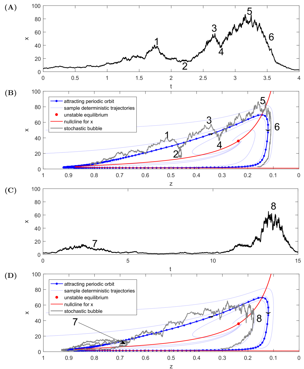
Fig 6. Schematic representation showing different phases and outcomes of stochastic bubbles for (4) with b = 0.42 , g = -0.04 , \sigma_x = 0.6 , \sigma_z = 0.0 . The bold blue line represents a deterministic stable orbit with blue dots at fixed time intervals. (A) and (B) Foreshocks {1/2} and {3/4} preceding the main crash {5/6} are clearly visible. The time intervals between the consecutive local peaks and corrections decrease as a result of at least two factors: first, until around z = 0.2 , the price x accelerates making it prone to take a time consuming detour for smaller x {2} that becomes less impactful compared to when x is larger {4}. (C) and (D) The noise can push the dynamics to enter the region where deterministic forces drag trajectories back to the region of small x , thus aborting the bubble {7} before it fully develops. The same kind of behaviour for higher x levels can shorten the life of a bubble in the regime close to the unstable fixed point where the price dynamics can oscillate temporarily before the main crash {8}.
