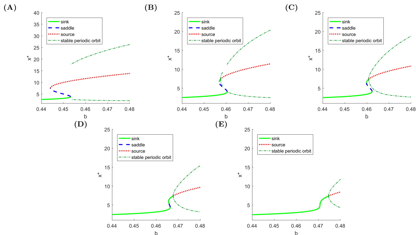
Fig 3. One parameter bifurcation diagrams for fixed g < 0 . (A) g = -0.067 , periodic orbits appear when a saddle collides with a sink, (B) g = -0.071 , periodic orbits appear via a Hopf bifurcation, exist until a homoclinic bifurcation occurs and then appear again when a saddle collides with a sink, (C) g = -0.072 , periodic orbits emerge from a Hopf bifurcation point, which occurs between two fold bifurcations, (D) g = -0.074 , the fold bifurcations are approaching each other, (E) g = -0.076 , only the Hopf bifurcation remains, from which periodic orbits appear.
