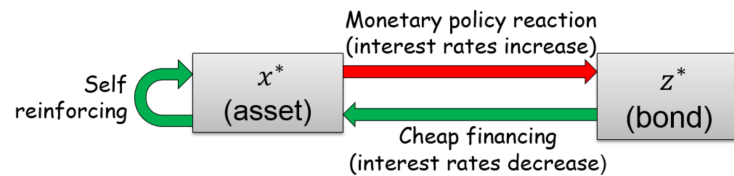
Fig 1. Schematic diagram showing the feedback loops governing the prices x(t) and z(t) for the model (1) of [10]. An increasing bond price means mechanically a lower interest rate and thus a lower borrowing cost, which favours further stock price increase (term e^{-bxz} with b > 0 ). A large stock price leads to a reaction of the central bank to increase the interest rates and thus decrease the bond price (term e^{-gx} with g < 0 ). A larger stock price is also assumed to feedback positively on itself (term e^{-bxz} with b > 0 ).
