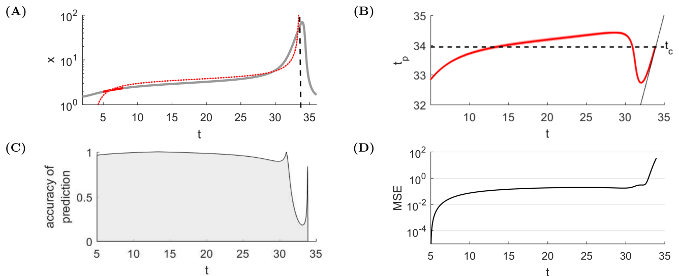
Fig 9. Sample application of the ghosts of finite-time singularities in the deterministic system (1) for parameters b = 0.42 and g = -0.04 . (A) Presentation of one fit (thin red line) for a small sample set representing current knowledge up to ‘present time’ t_2 = 8 (bold red) compared with the true price trajectory (grey). The predicted time of the crash (i.e. where the finite-time singularity occurs in (12)—indicated by the dashed black line) is very close to the peak of the bubble and therefore provides an accurate forecast. (B) Time t_p of the predicted crash (red) as a function of the ‘present’ time t until which we assume we have knowledge of the price dynamics, compared with the exact crash time t_c . We apply here a sliding window of arbitrary length w = 3 . The following section explains the methodology that we follow to choose the optimal window length. When the bubble starts to grow rapidly (around t = 30 ), the predicted crash time t_c decreases towards the present time t and, as t increases, t_p remains close to t as can be seen by the line t_p = t (solid black). The price acceleration thus tends to induce the calibration to believe that the crash is looming, exaggerating the imminence of the danger. (C) Accuracy of crash prediction measured by 1 - |t_c - t_p|/|t_c - t_2| . The prediction accuracy is remarkably high already very far from the crash, and does not improve significantly over most of the lifetime of the bubble. However, when time passes 30, the accuracy deteriorates dramatically. It is caused by the fact that the predictions are based on the normal form truncation close to equilibrium. This is not the case after time 30 when the system grows exponentially. In other words, the prediction system develops a myopic optical illusion when approaching close to the end of the bubble. (D) Mean Square Error for the fitted function (12). When the bubble starts to rise rapidly, the MSE increases very quickly, confirming the loss of reliability of the prediction.
