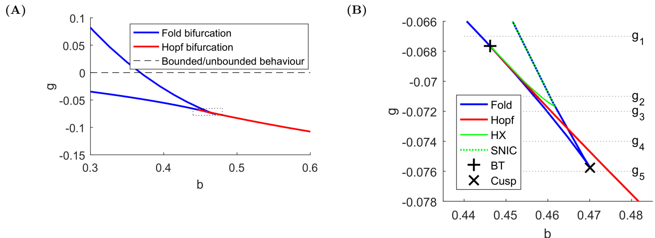
Fig 2. Two-parameter bifurcation diagram. (A) Macroscopic view, (B) zoom-in on the marked rectangle in Panel (A). The dotted lines represent certain bifurcation paths, which are shown in Fig 3. BT means Bogdanov-Takens point. Bifurcations are computed using XPPAUT [31].
