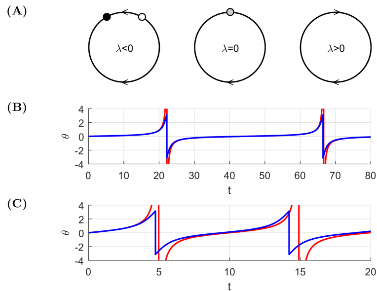
Fig 8. Example of ghosts of finite-time singularities and real finite-time singularities. (A) Schematic bifurcation diagram of the flow of system (6). For \lambda < 0 , there are two equilibria—one stable (black) and one unstable (white), for \lambda = 0 , a saddle-node bifurcation occurs and for \lambda > 0 (if we allow discontinuities in the solutions), one can observe periodic orbits between -\pi and \pi . In the two-dimensional case, discontinuities are not necessary to obtain a periodic behaviour. Panels (B) and (C) show the sample solutions for systems (6) and (9). The blue curve is the original accurate solution of the full dynamics, where no finite-singularity occurs. The red one is the approximation based on the saddle-node normal form. In the solution based on normal form, there are finite-time singularities whereas, in the original one, bubbles and crashes are bounded. The jump behaviour exhibited by the exact solution of the full system is called the ghost of the singularity associated with the normal form approximation. Parameter values are: (B) \lambda = 0.01 and (C) \lambda = 0.2 .
