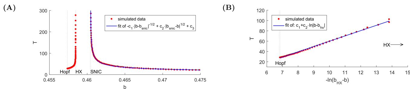
Fig 4. Analysis of the orbit periods for g_2 = -0.071 . (A) Scenario 1 of approaching HX (left series of dots) and scenario 2 of approaching SNIC (right series of dots fitted by expression (3)), (B) Scenario 1 of approaching HX: logarithmic transformation of the distance from the bifurcation point approximated by a linear function.
