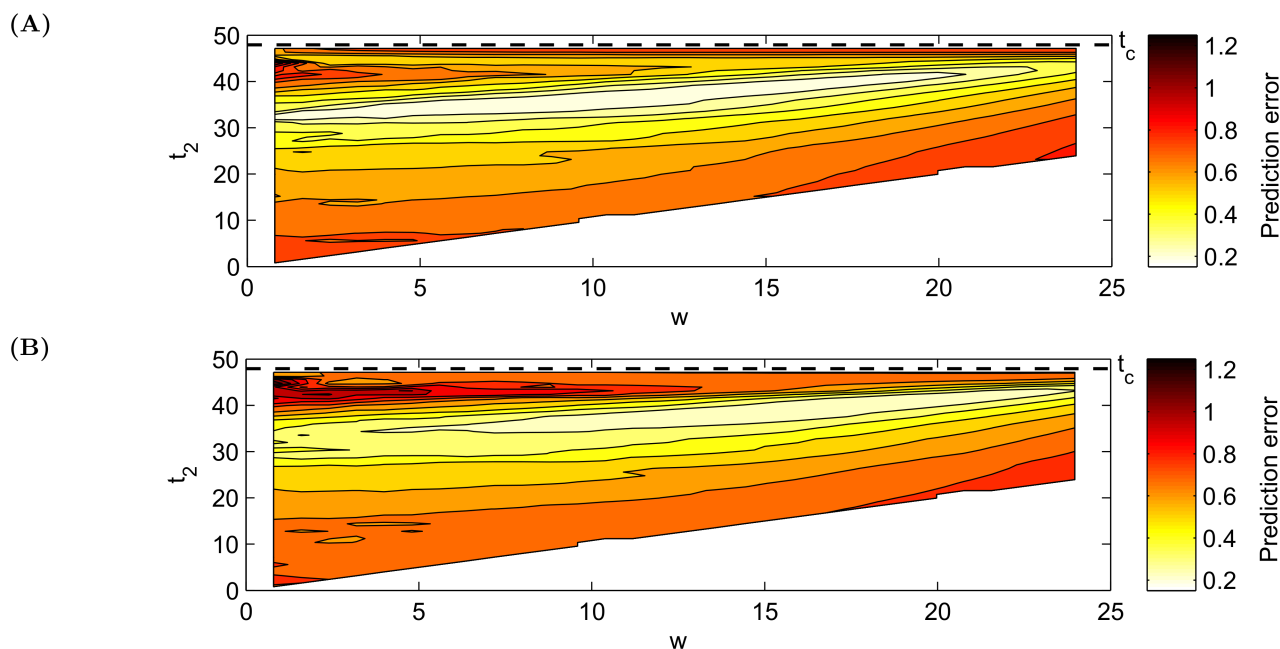
Fig 10. Dependence of the prediction error \frac{|t_c - t_p|}{|t_c - t_2|} as a function of window size w and end t_2 of window. (A) For \sigma_x = 0.2 , the optimal window length is around 10. (B) For \sigma_x = 0.4 , the optimal window length is around 15. The parameters of the model are b = 0.42 , g = -0.04 , \sigma_z = 0.01 , \delta(W_t^{(1)}, W_t^{(2)}) = 50\% . For both selected window sizes, the error just before the time of a crash t_c does not significantly differ in comparison to larger w 's and, moreover, the smaller w is, the faster the system responds to new information. There is thus a trade-off between responsive adaptation of the fits and error size.
