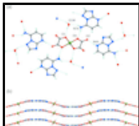
Fig. 2. View along the a -axis showing the formation of the hydrogen bonded (thin blue lines) layer (a); view of the packing of the layers (b).
