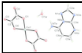
Fig. 1. ORTEP representation of the asymmetric unit of the title compound, showing the atom labels and displacement ellipsoids drawn at the 50% probability level.
