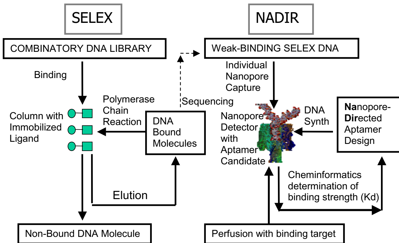
Figure 12 The determination of aptamers can be done (or initiated) via Systematic Evolution of Ligands by Exponential Enrichment (SELEX), as shown schematically on the left. What is proposed here is a linkage to a nanopore-detector directed (NADIR) search for aptamers that is based on bound-state lifetime measurements. NADIR complements and augments SELEX in usage: SELEX can be used to obtain a functional aptamer, and NADIR used for directed modifications (for stronger binding affinity, for example).
