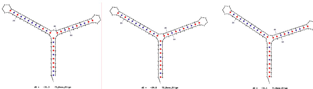
Figure 13 Shown are Y-shaped aptamers that have shown they have capture states with the desired blockaded toggling.
