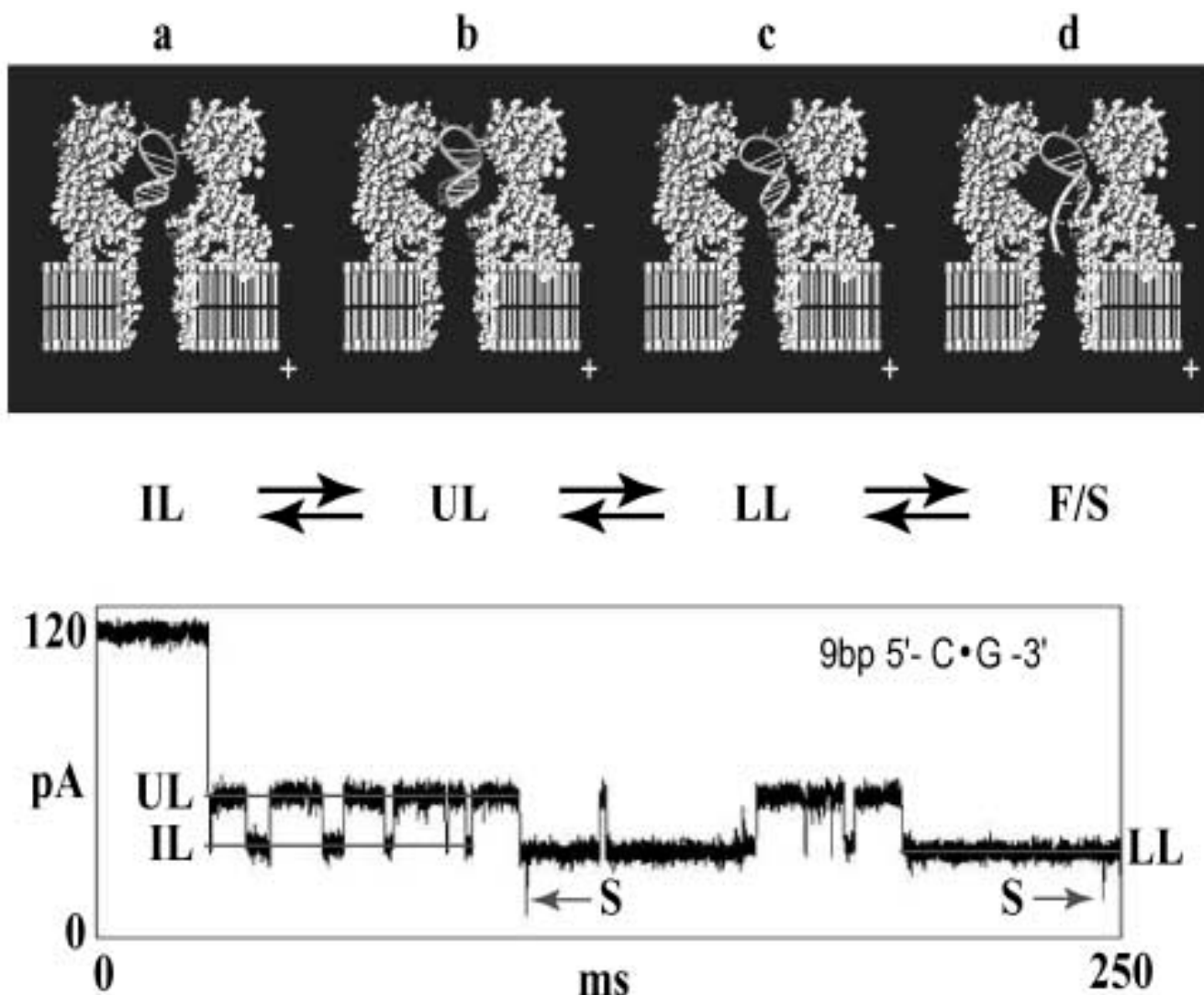
Figure 5 Shows the nine base pair DNA hairpin blockade mechanism (from [11]). When a 9 bp DNA hairpin initially enters the pore, the loop is perched in the vestibule mouth and the stem terminus binds to amino acid residues near the limiting aperture. This results in the IL conductance level. When the terminal base pair desorbs from the pore wall, the stem and loop may realign, resulting in a substantial current increase to UL. Interconversion between the IL and UL states may occur numerous times, or UL may convert to the LL state. The LL state corresponds to binding of the stem terminus to amino acids near the limiting aperture but in a different manner from IL. From the LL bound state, the duplex terminus may fray with rapid extension and capture of one strand in the pore constriction (denoted F/S).
