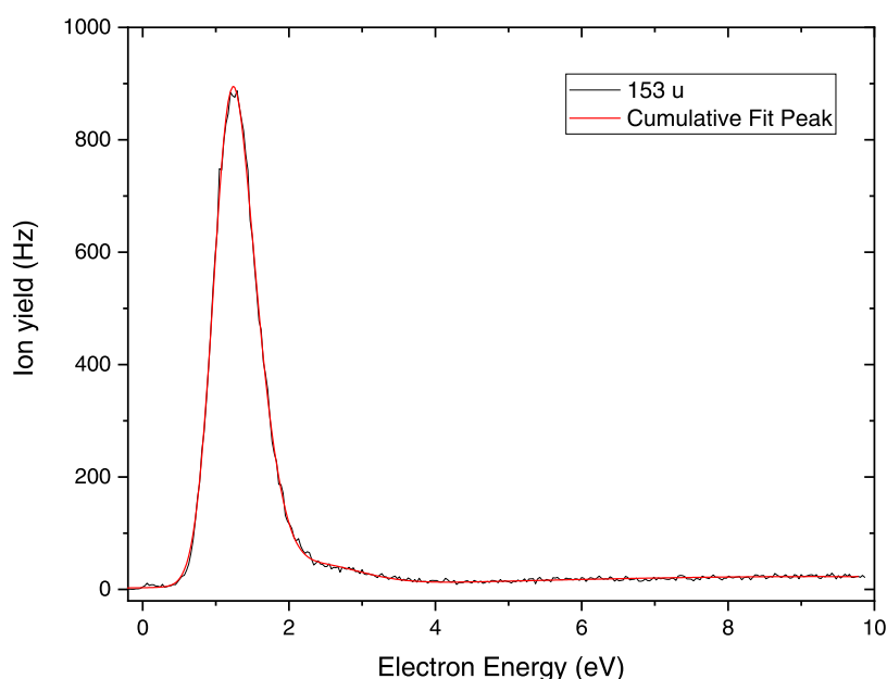
Figure 3. Anion efficiency curve for the formation of \text{C}_4\text{H}_{10}\text{PO}_4^- upon electron attachment to tetra-Et-dCDP. Black line, experimental data; red line, cumulative peak fit.
