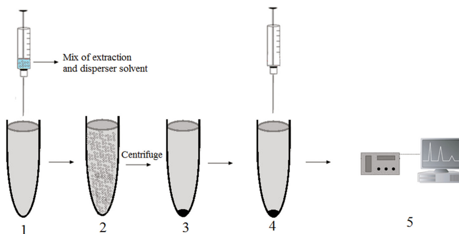
Fig. 2 – Different steps of dispersive liquid–liquid phase microextraction: (1) rapid injection of a mixture of disperser and extraction solvent into the aqueous solution; (2) formation of a cloudy solution; (3) sedimentation of the extraction solvent after centrifugation; (4) removal of sedimented phase; and (5) instrumental analysis.
