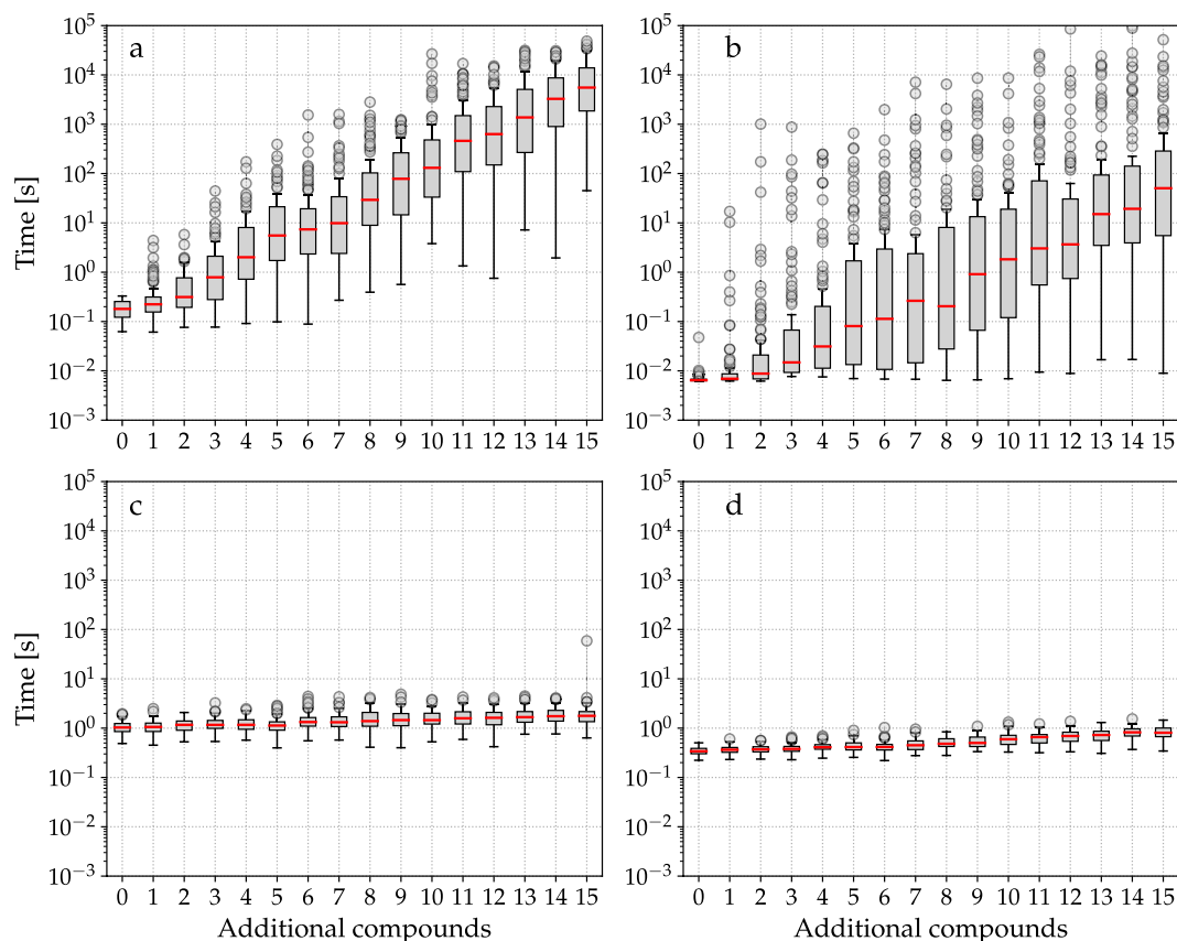
Figure 3. Searching times required to find a metabolic pathway considering a growing number of compounds added to the minimum set of available ones. (a) BFS; (b) DFS; (c) EvoMS; (d) PhDSeeker. Red line denotes the median, and circles indicate outliers.
