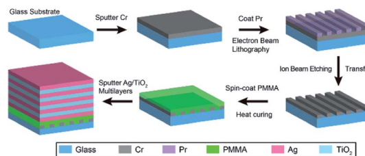
Fig. 3 Schematic of the fabrication process of the planar lithography objective lens and mask.
